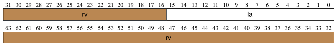
Figure 11-36. Layout of proc_n_cache_info2 Return Value
