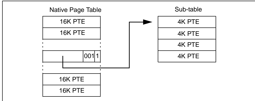
Figure 5-2. Subpaging
