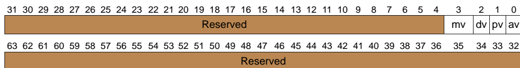
Figure 11-75. Layout of TR_valid Return Value
