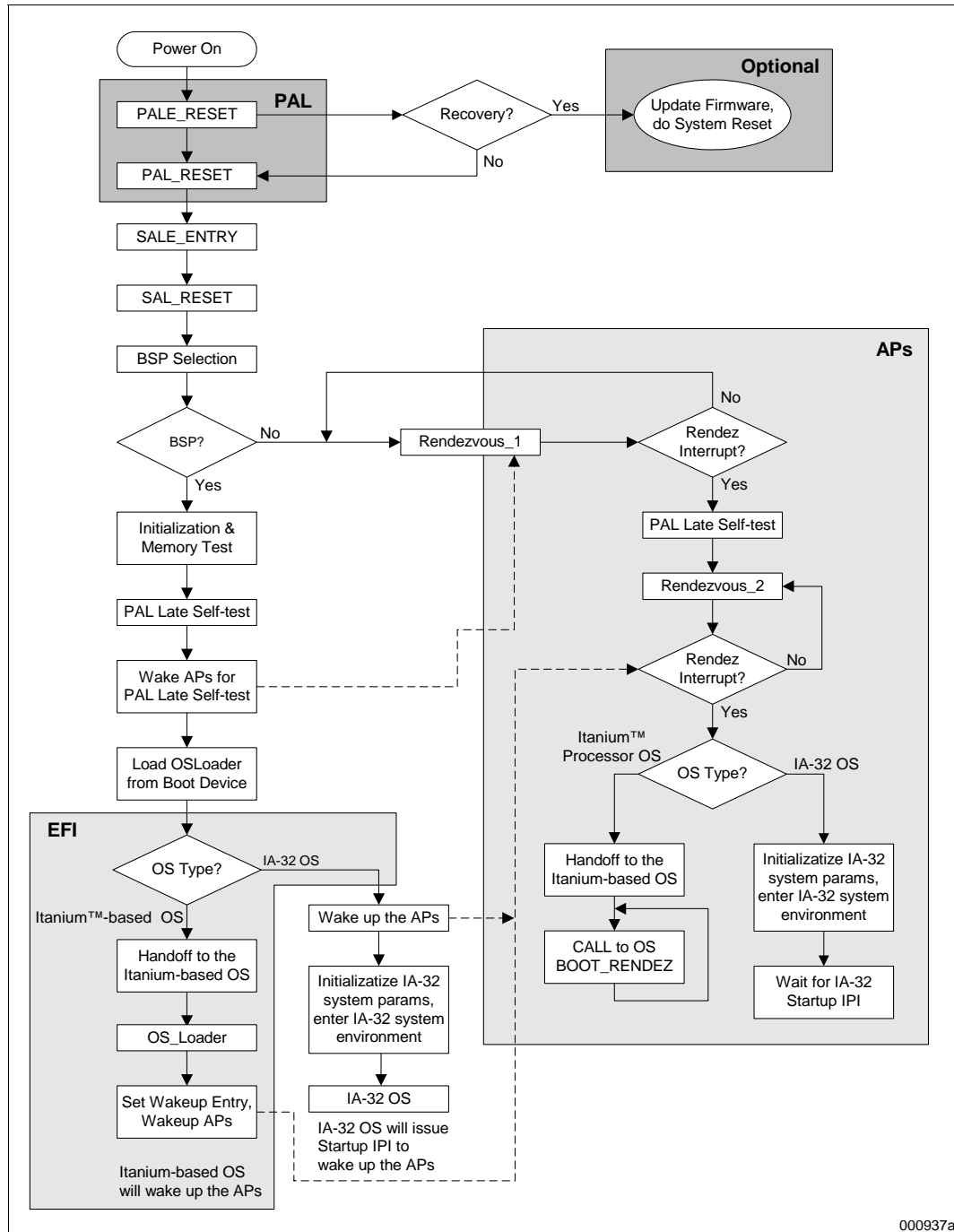
Figure 13-2. Control Flow of Boot Process in a Multiprocessor Configuration
