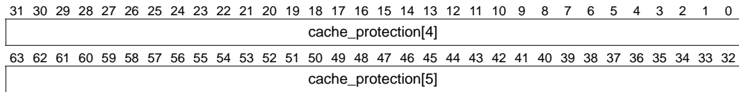
Figure 11-32. config_info_3 Return Value
