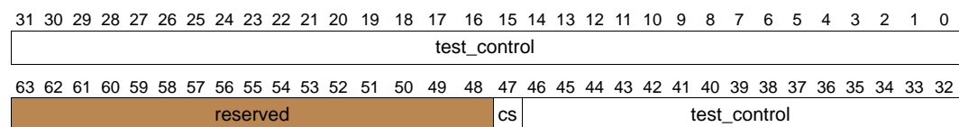
Figure 11-11. Self-test Control Word
