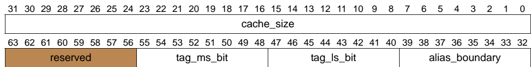
Figure 11-29. config_info_2 Return Value
