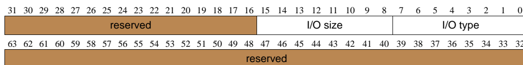
Figure 11-39. I/O Size and Type Information Layout
