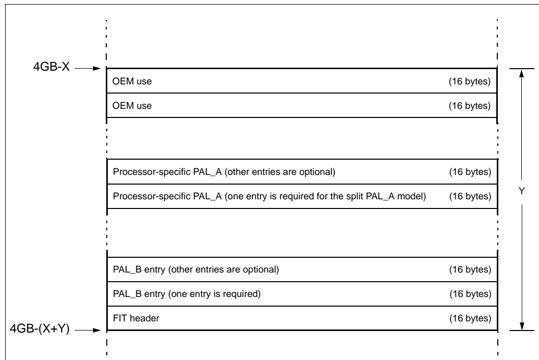
Figure 11-6. Firmware Interface Table
