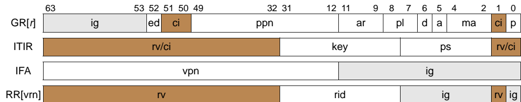
Figure 4-5. Translation Insertion Format
