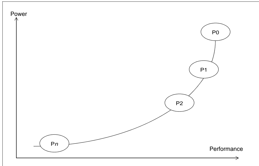
Figure 11-20. Power and Performance Characteristics for P-states
