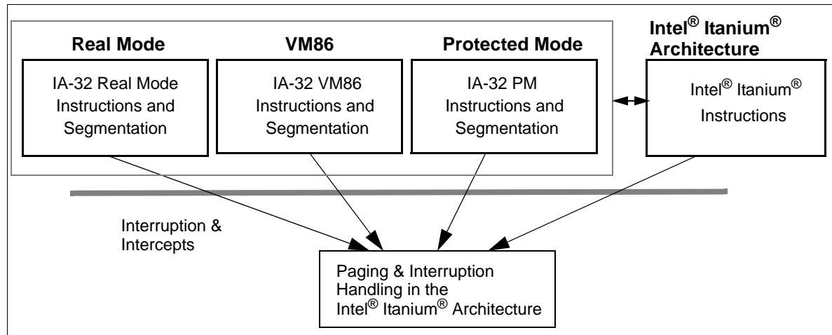
Figure 2-2. Intel® Itanium® System Environment
