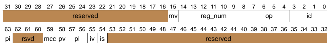
Figure 11-49. reg_file_check Layout
