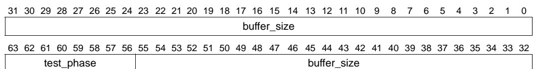
Figure 11-69. Layout of test_info Argument
