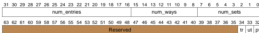
Figure 11-72. Layout of tc_info Return Value
