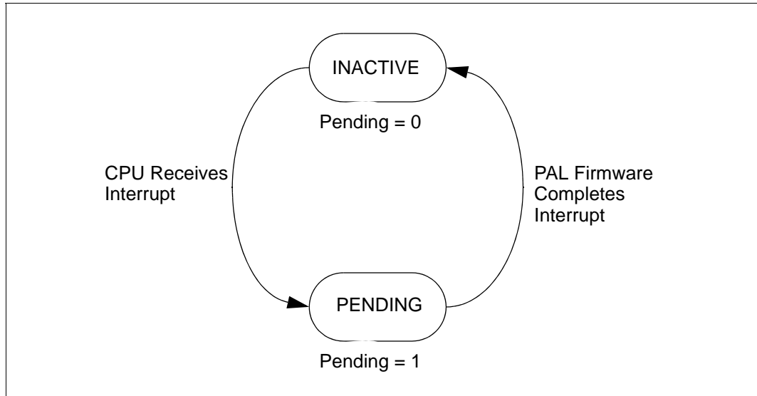
Figure 5-5. External Interrupt States
