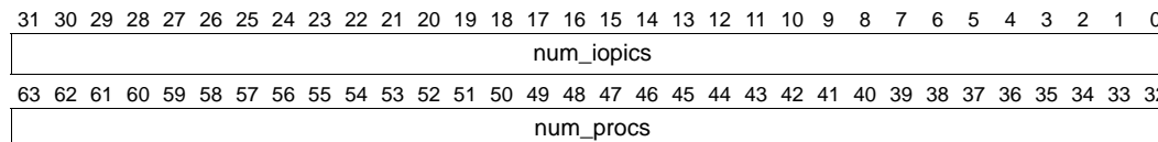
Figure 11-38. Layout of platform_info Input Parameter
