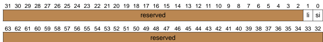
Figure 11-68. Layout of hints Return Value
