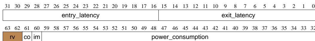
Figure 11-40. Layout of power_buffer Return Value
