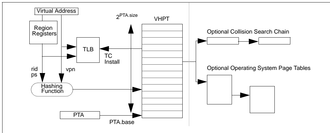
Figure 4-9. Virtual Hash Page Table (VHPT)
