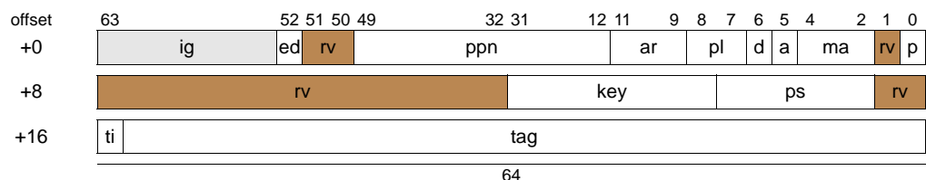
Figure 4-12. VHPT Long Format
