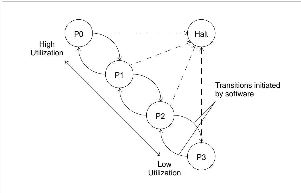
Figure 11-21. Example of a P-state Transition Policy
