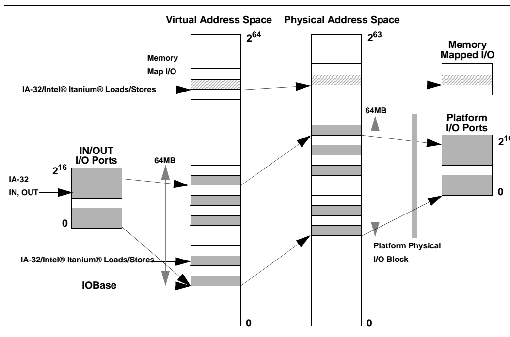
Figure 10-6. I/O Port Space Model
