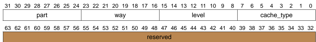
Figure 11-34. Layout of line_id Return Value
