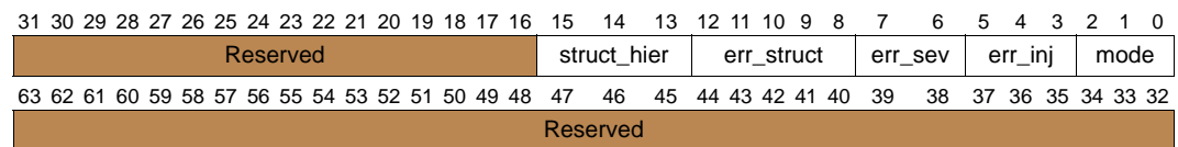
Figure 11-51. err_type_info
