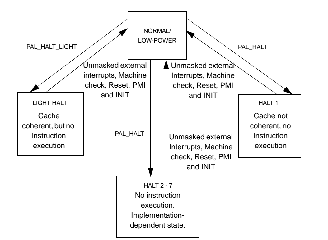
Figure 11-19. Power States
