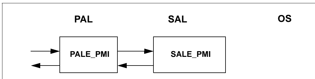
Figure 11-18. PMI Entrypoints
