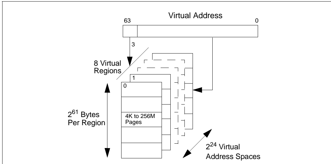
Figure 4-1. Virtual Address Spaces
