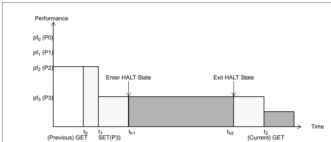
Figure 11-23. Interaction of P-states with HALT State
