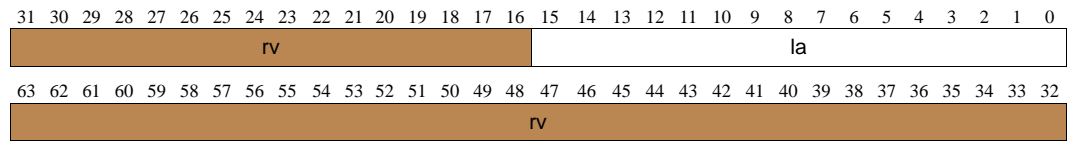
Figure 11-43. Layout of proc_n_log_info2 Return Value
