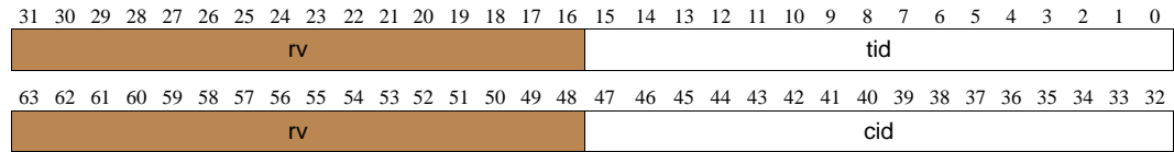
Figure 11-35. Layout of proc_n_cache_info1 Return Value
