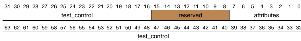
Figure 11-70. Layout of test_param Argument
