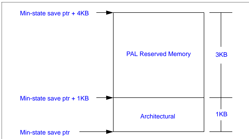
Figure 11-13. Processor Min-state Save Area Layout
