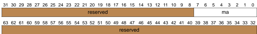
Figure 11-64. Layout of attrib Return Value
