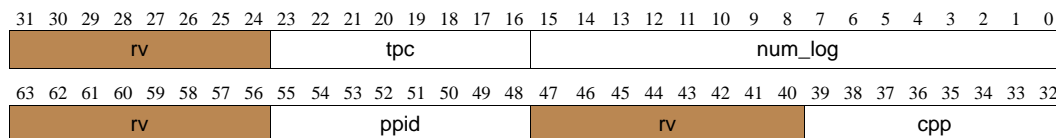
Figure 11-41. Layout of log_overview Return Value
