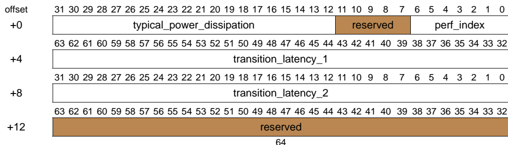
Figure 11-66. Layout of pstate_buffer Entry
