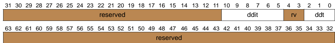
Figure 11-67. Layout of dd_info Parameter
