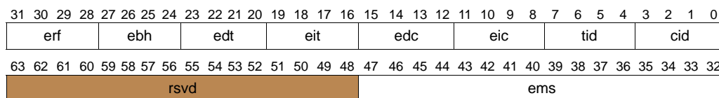
Figure 11-45. level_index Layout
