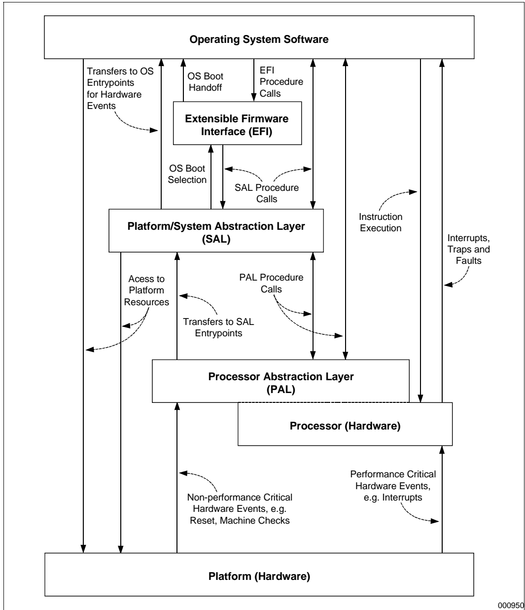
Figure 13-1. Firmware Model
