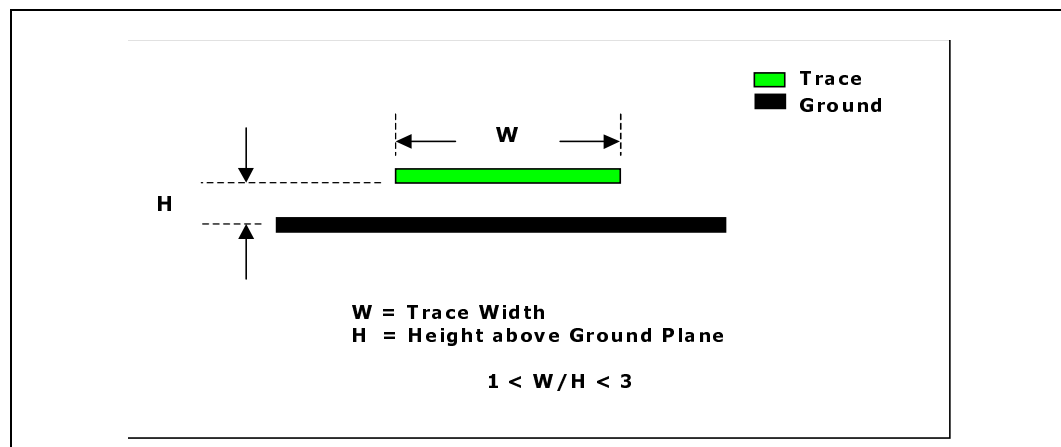
Figure 5. Trace Geometry
