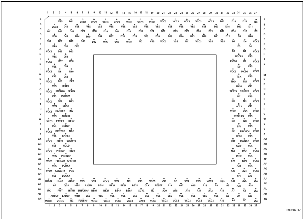
Figure 17. 320-Pin Socket 5
