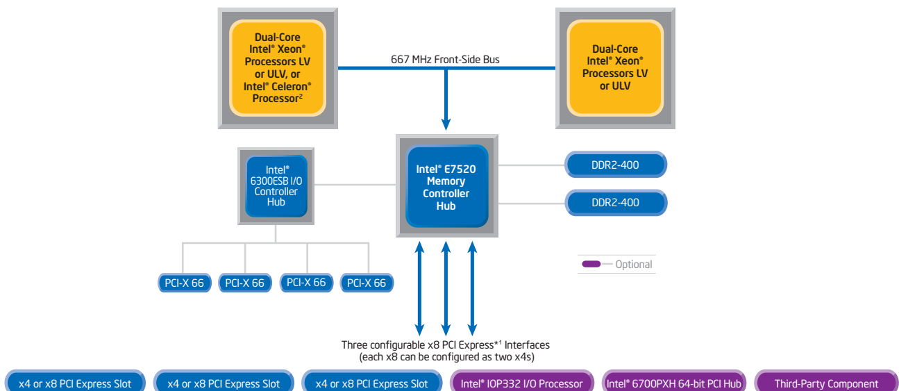
Figure 1: Intel® E7520 chipset with two Dual-Core Intel® Xeon® processors LV or ULV, or Intel® Celeron® processors 1.66 GHz and 1.83 GHz
