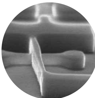
Intel 30nm Tri-gate Transistor
