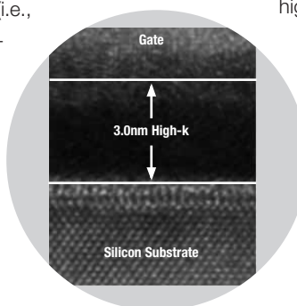
Future High-k Dielectric for Reduced Gate Leakage
