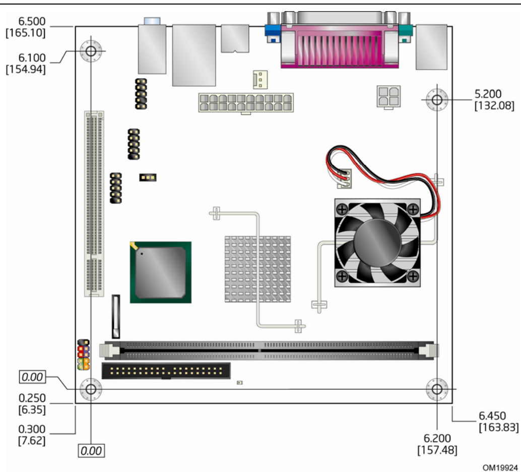
Figure 11. Board Dimensions
