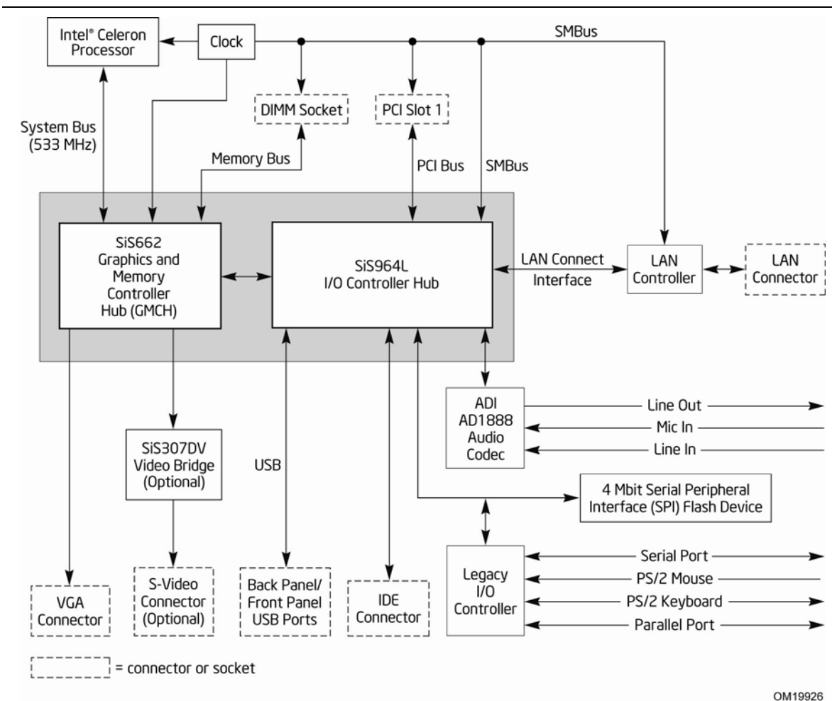
Figure 2. Block Diagram
