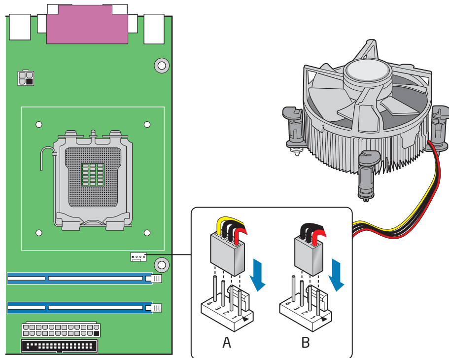
Figure 12. Connecting the Processor Fan Heat Sink Cable to the Processor Fan Header
