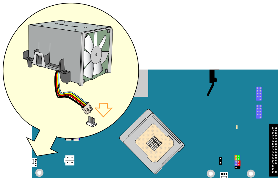
Figure 12. Connecting the Processor Fan Heat Sink Cable to the Processor Fan Connector
