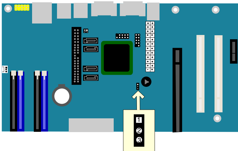
Figure 24. Location of the BIOS Configuration Jumper
