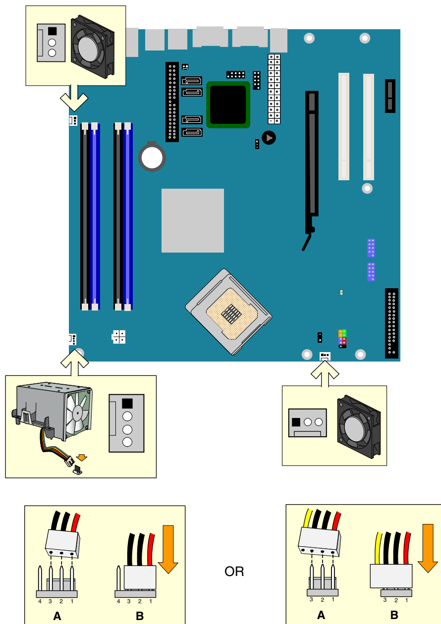
Figure 21. Location of Fan Headers
