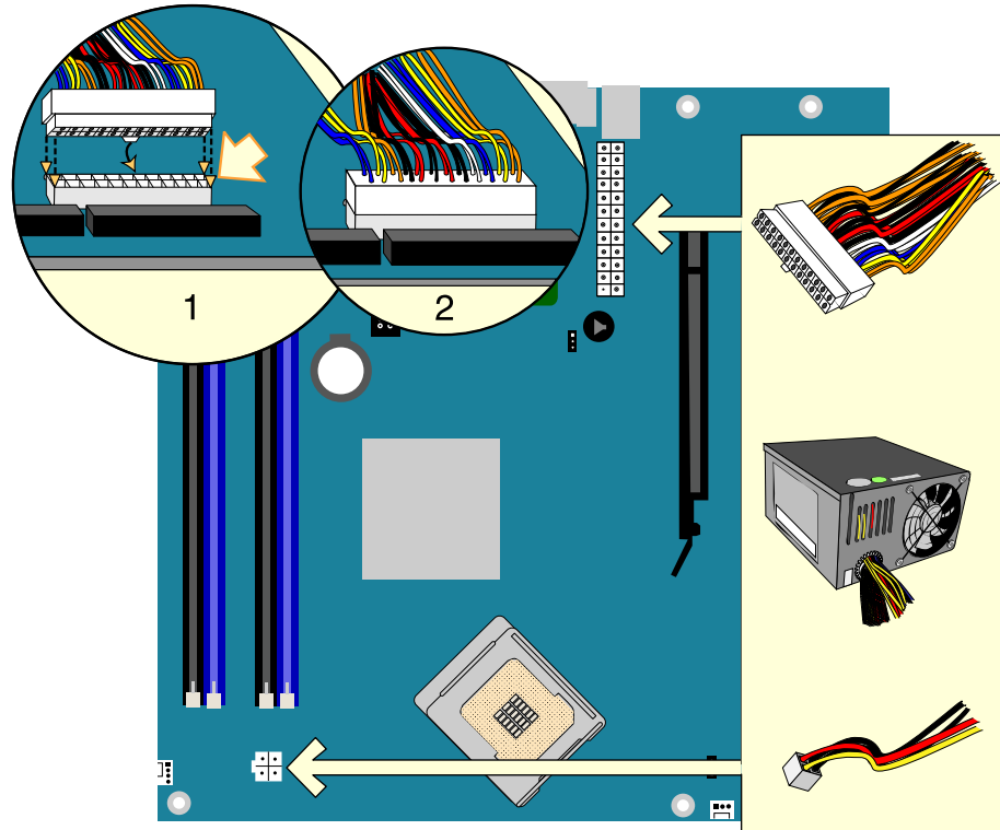
Figure 22. Connecting Power Supply Cables
