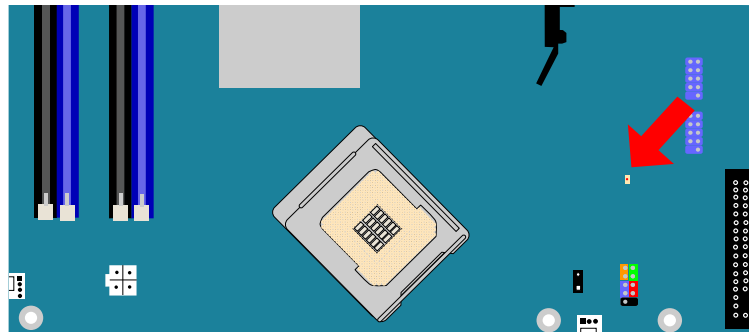
Figure 3. Location of Standby Power Indicator
