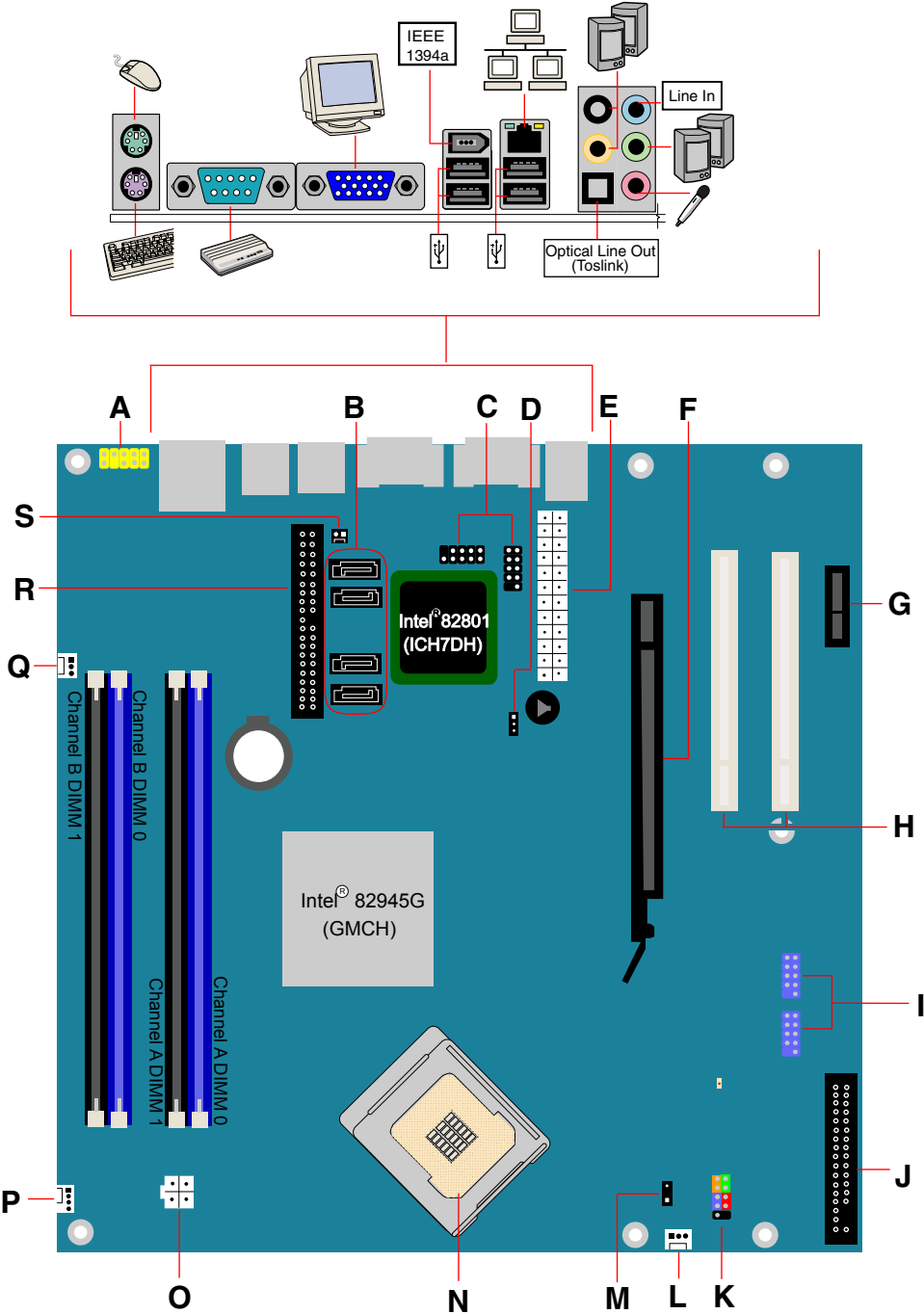
Figure 1. Desktop Board D945GBO Components
