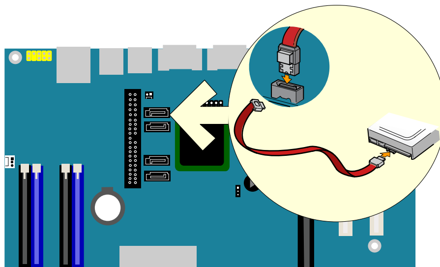
Figure 19. Connecting a Serial ATA Cable
