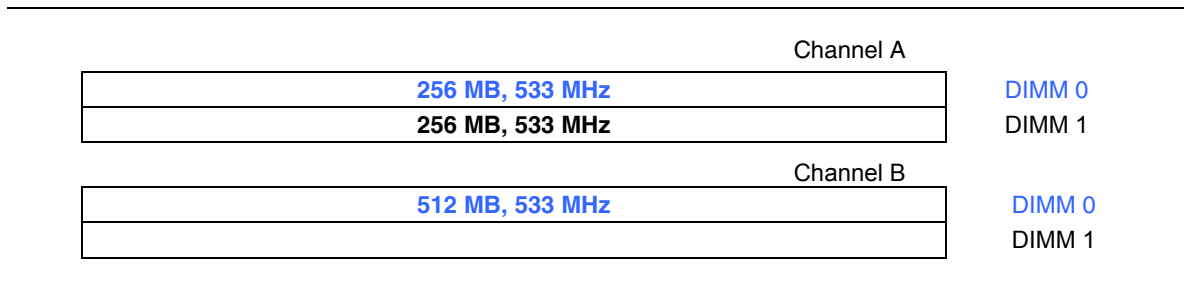
Figure 15. Dual Configuration Example 3
