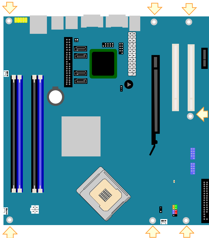
Figure 5. Desktop Board D945GBO Mounting Screw Hole Locations
