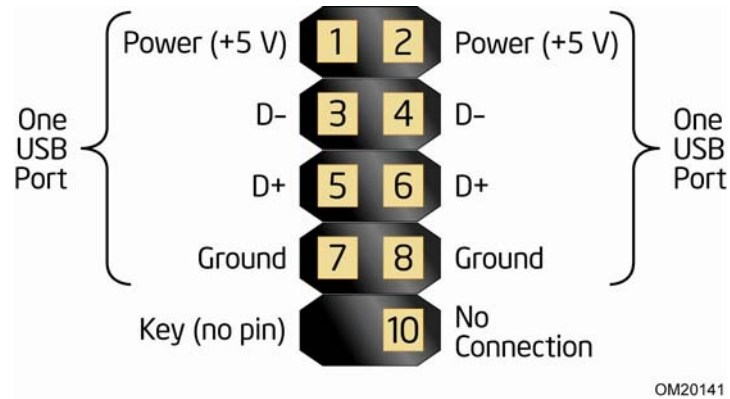
Figure 11. Connection Diagram for Front Panel USB Headers
