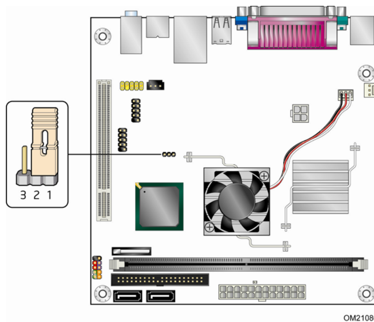
Figure 12. Location of the Jumper Block
