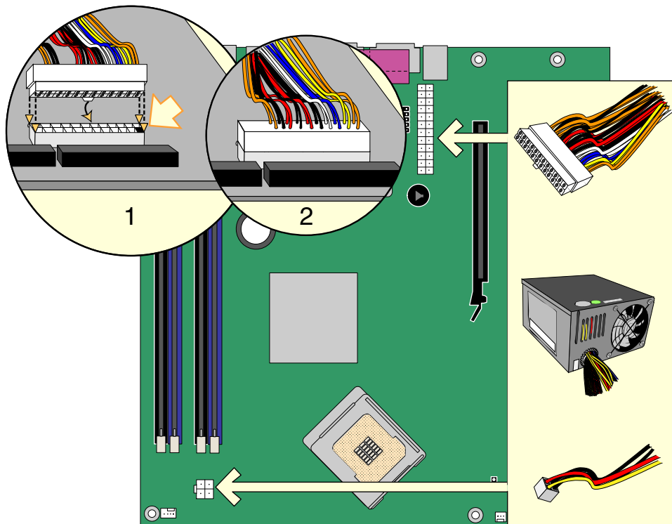
Figure 23. Connecting Power Supply Cables
