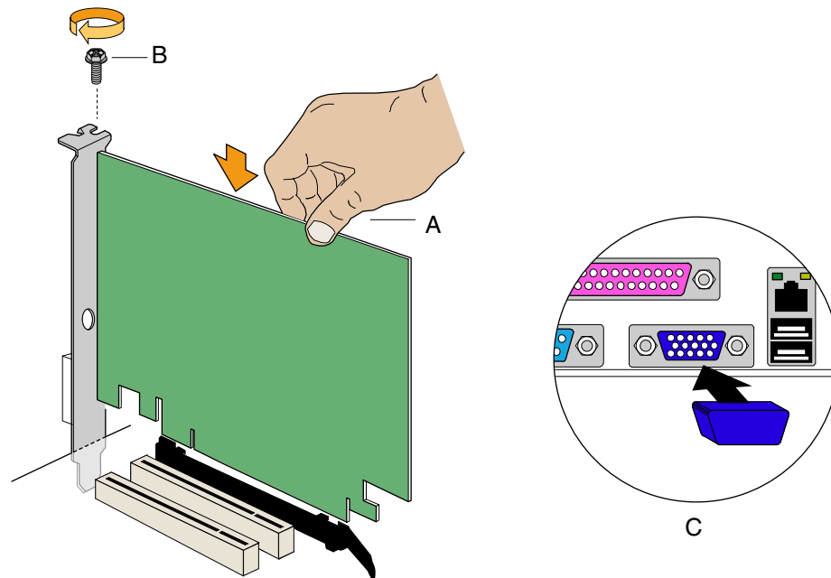
Figure 17. Inserting a PCI Express x16 Card and Covering the Back Panel VGA Port
