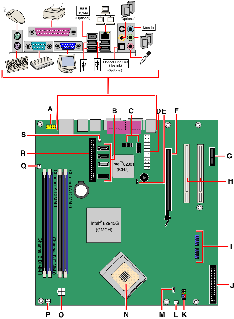
Figure 1. Desktop Board D945GCZ Components
