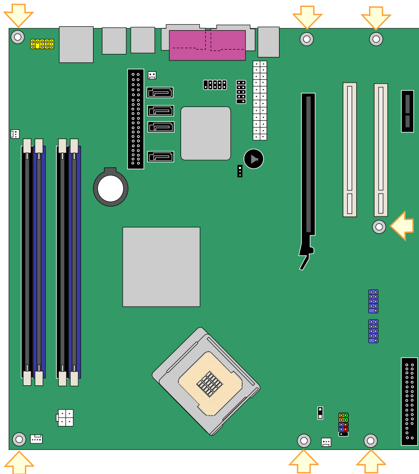
Figure 5. Desktop Board D945GCZ Mounting Screw Hole Locations
