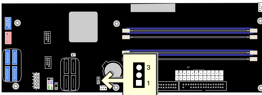
Figure 30. Location of the BIOS Configuration Jumper Block
