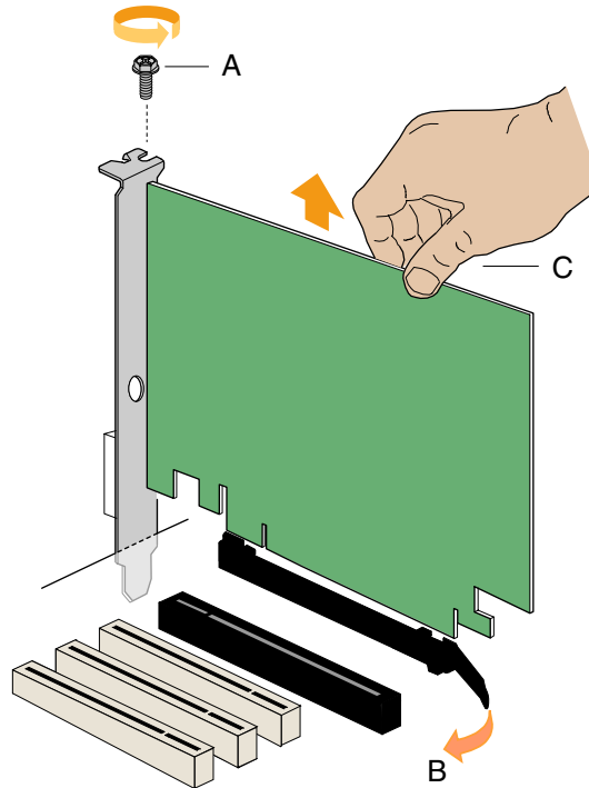
Figure 19. Removing the PCI Express x16 Card
