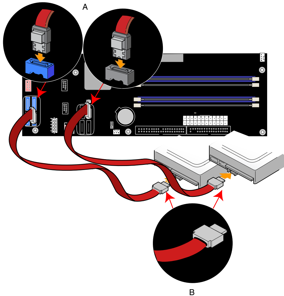
Figure 21. Connecting Serial ATA Cables
