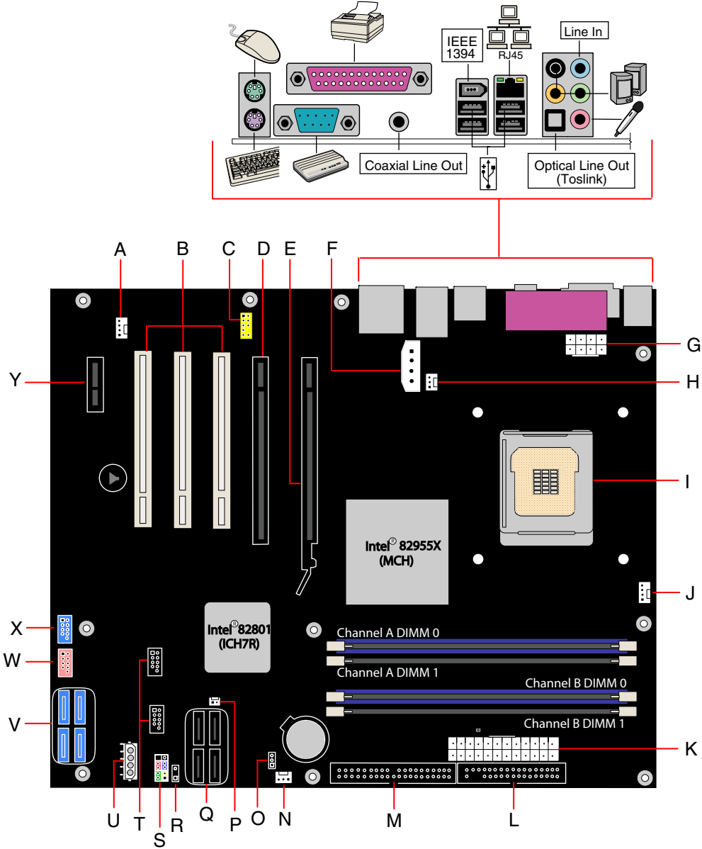
Figure 1. Desktop Board D955XBK Components
