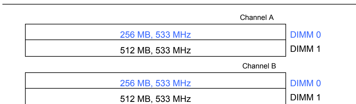
Figure 14. Dual Configuration Example 2
