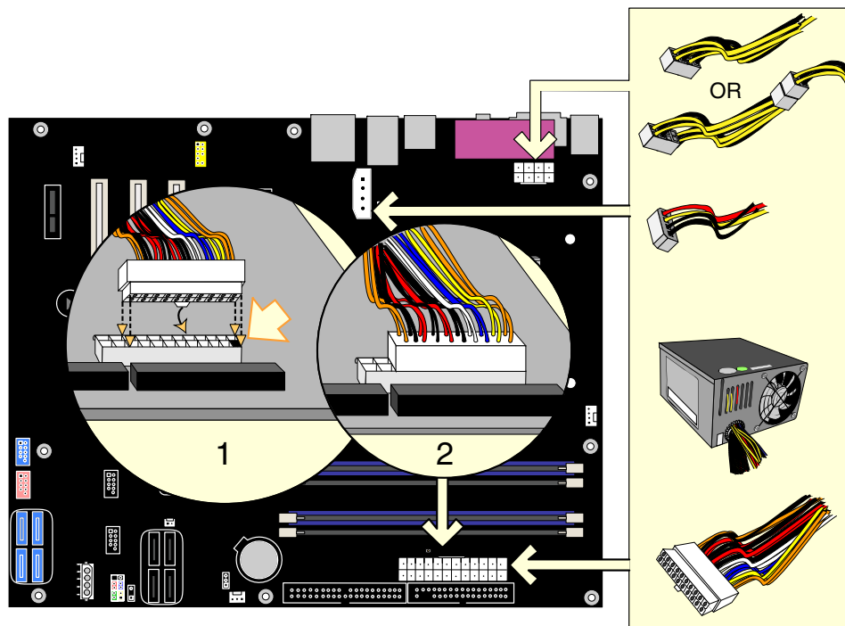
Figure 27. Connecting 2x10 Power Supply Cables
