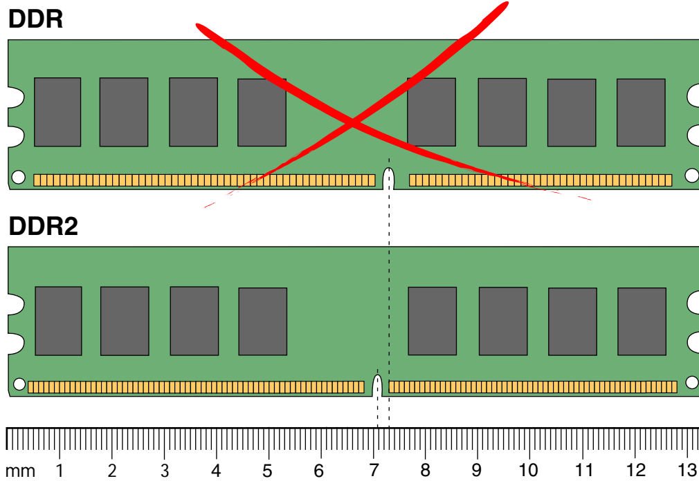
Figure 16. Use DDR2 DIMMs
