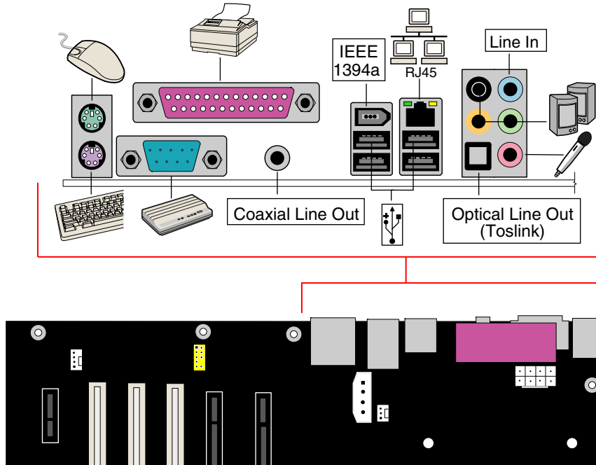
Figure 31. Back Panel Connectors
