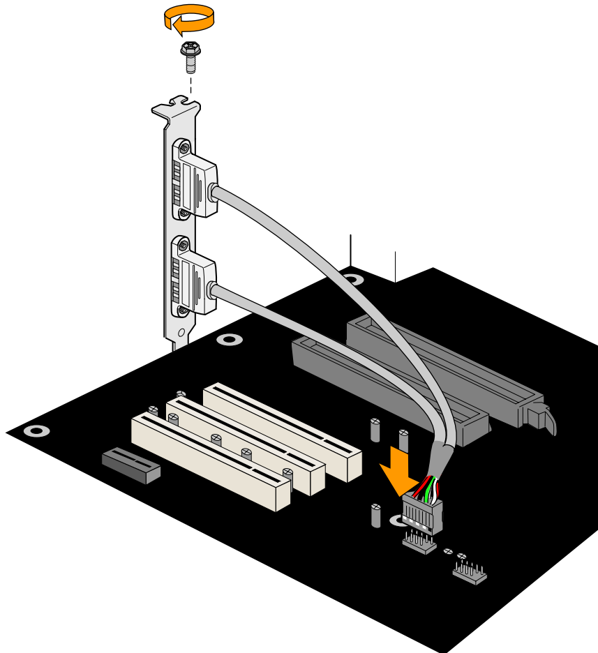
Figure 23. Connecting the Rear Panel USB 2.0 Adapter
