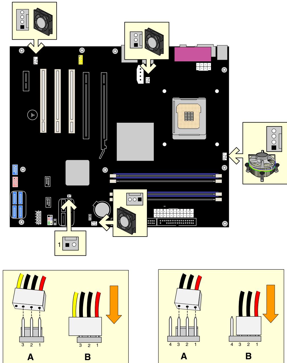
Figure 25. Location of Fan Headers
