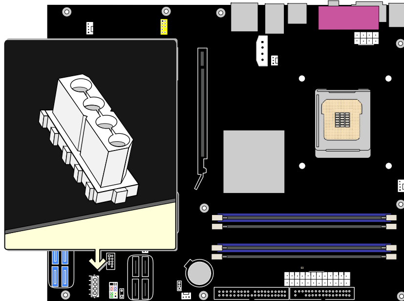
Figure 26. Auxiliary Power Output Connector
