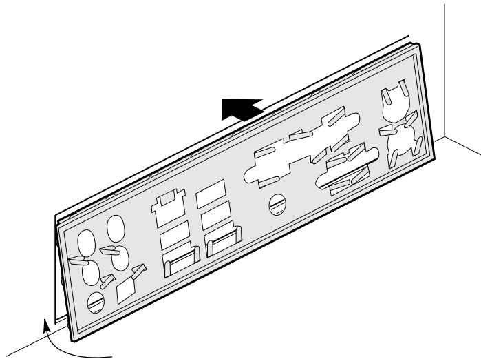
Figure 4. Installing the I/O Shield
