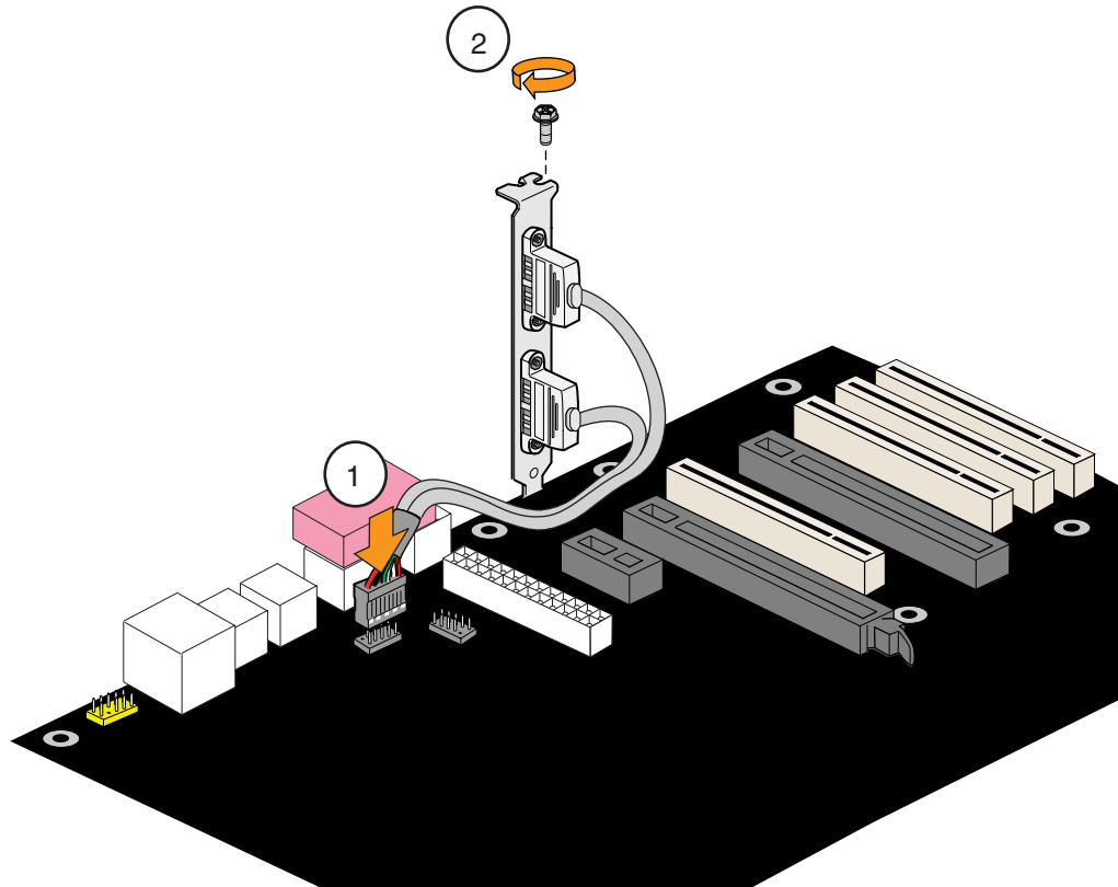
Figure 23. Connecting the Rear Panel Hi-Speed USB 2.0 Adapter
