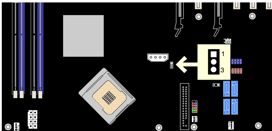
Figure 30. Location of the BIOS Configuration Jumper Block
