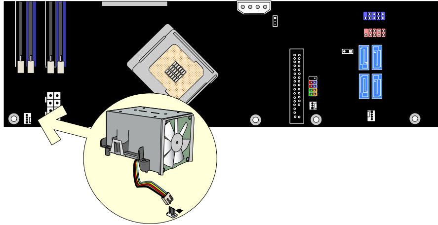
Figure 12. Connecting the Processor Fan Heat Sink Cable to the Processor Fan Header
