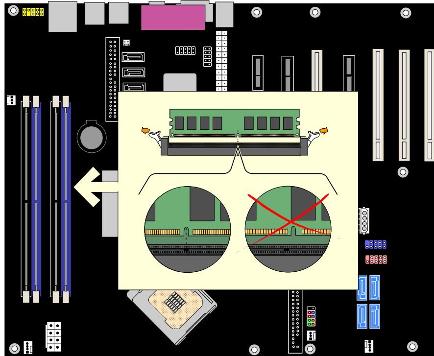
Figure 17. Installing a DIMM
