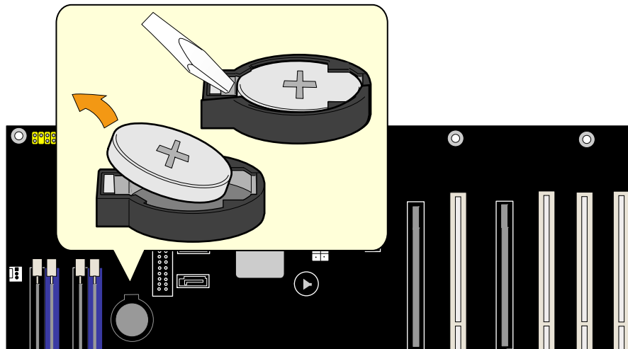
Figure 32. Removing the Battery
