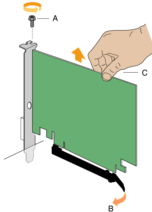
Figure 19. Removing the PCI Express x16 Card
