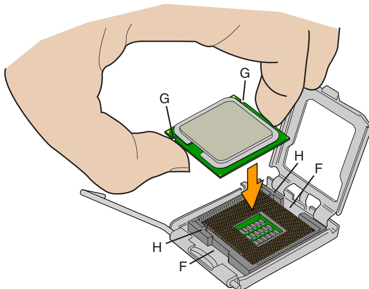
Figure 10. Install the Processor
