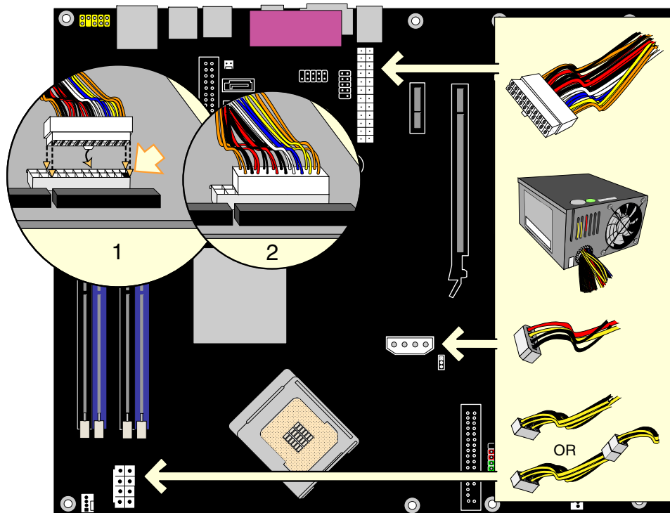
Figure 27. Connecting 2x10 Power Supply Cables
