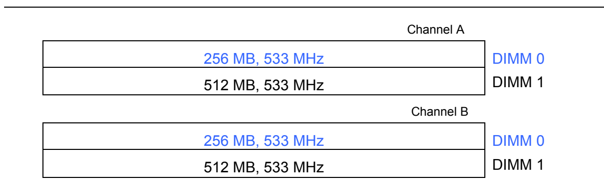
Figure 14. Dual Configuration Example 2
