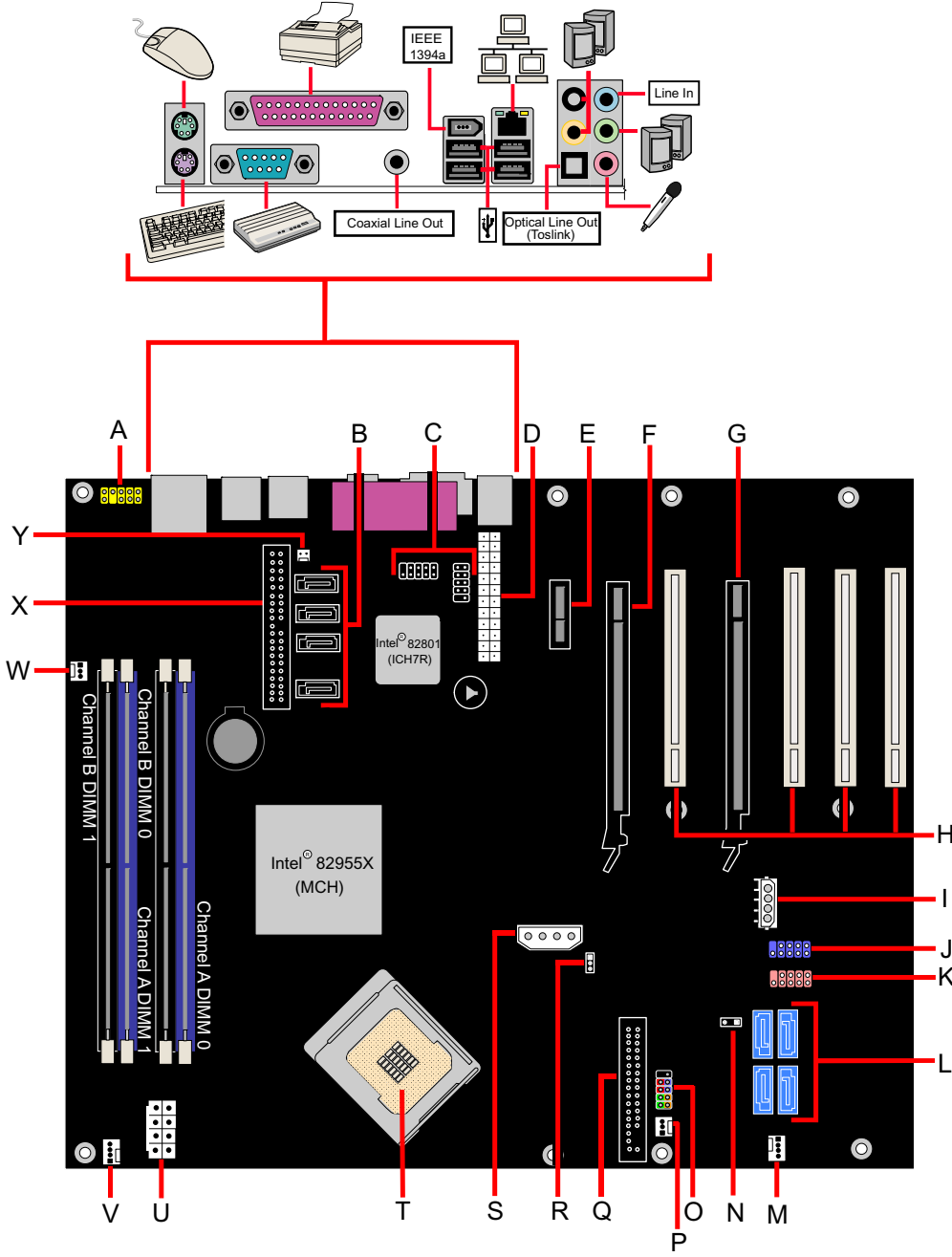
Figure 1. Desktop Board D955XCS Components
