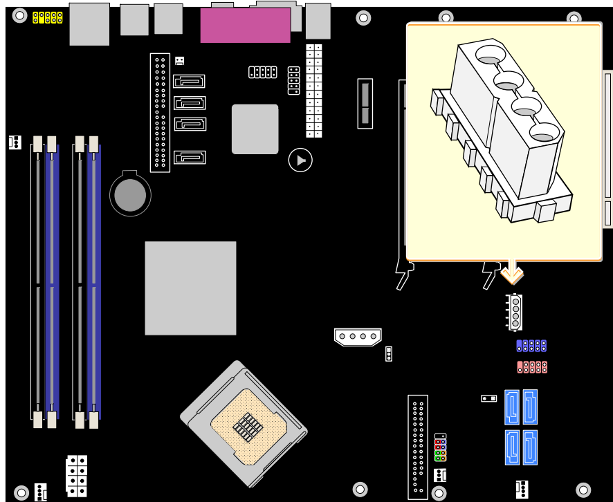
Figure 26. Auxiliary Power Output Connector
