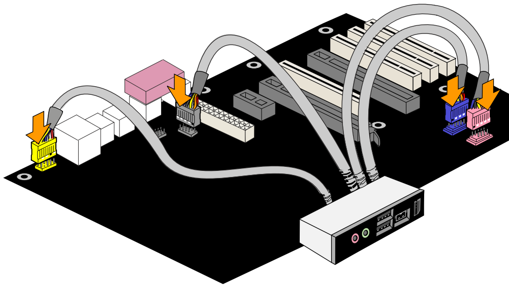
Figure 24. Connecting the Front Panel USB/IEEE 1394/Audio Cables
