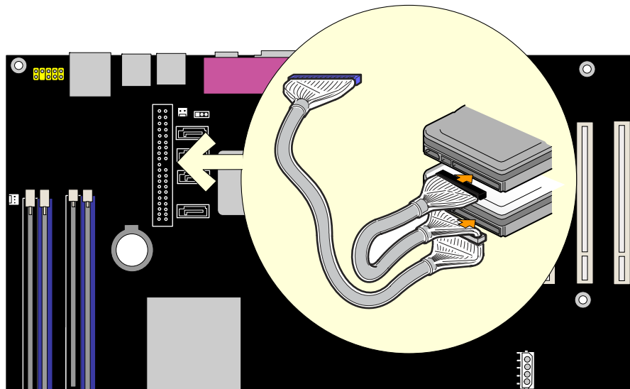
Figure 20. Connecting the IDE Cable
