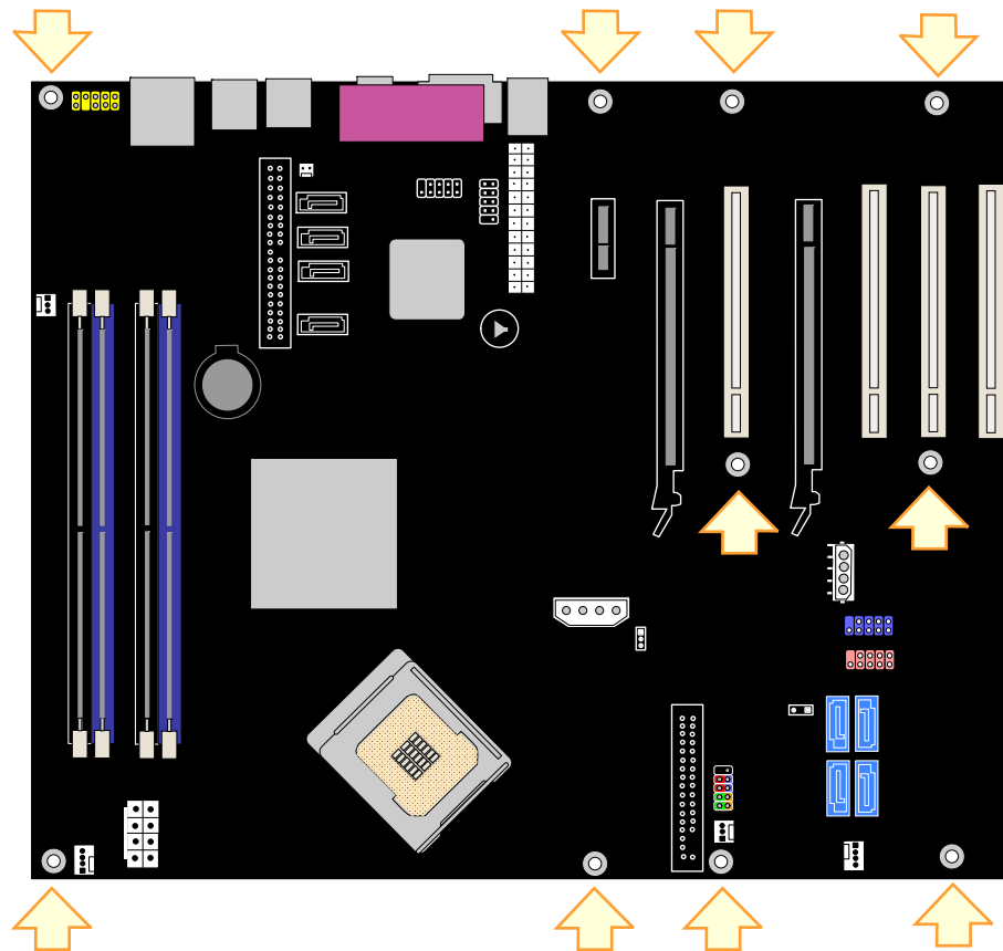
Figure 5. Location of Mounting Screw Holes
