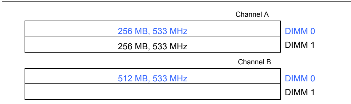
Figure 15. Dual Configuration Example 3
