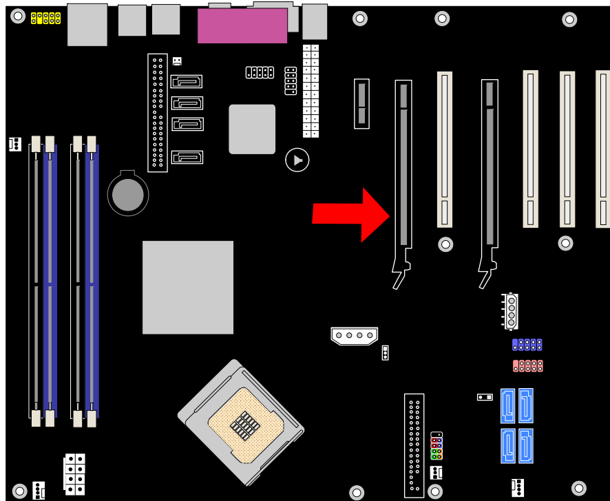
Figure 18. Slot to Use for One Video Card
