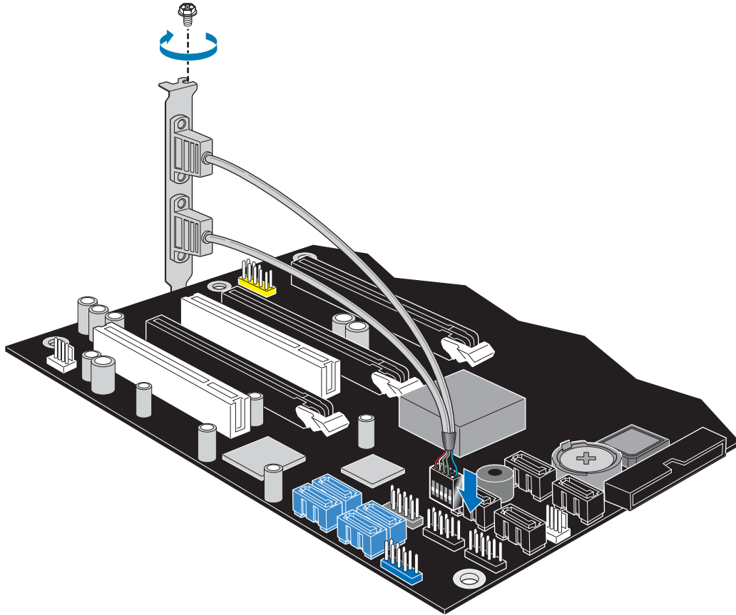
Figure 23. Connecting the Rear Panel USB 2.0 Adapter
