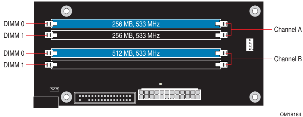
Figure 15. Dual Channel Memory Configuration Example 3
