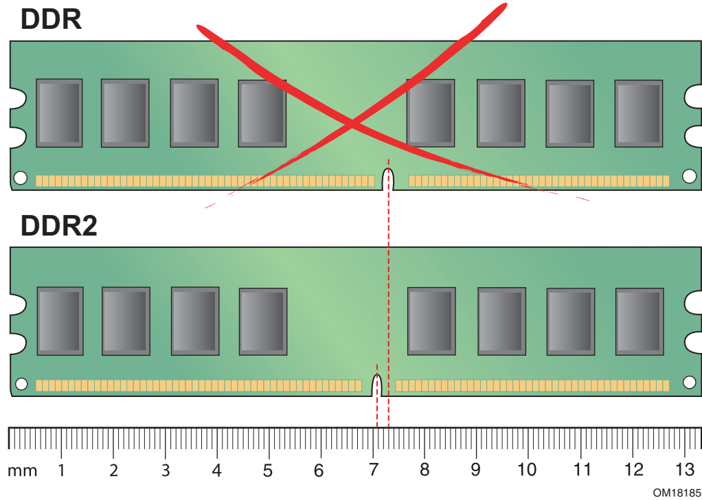
Figure 16. Use DDR2 DIMMs
