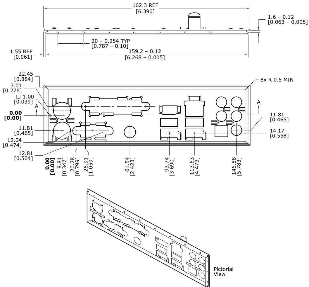
Figure 26. I/O Shield Dimensions for Boards with the 8-Channel (7.1) Audio Subsystem
