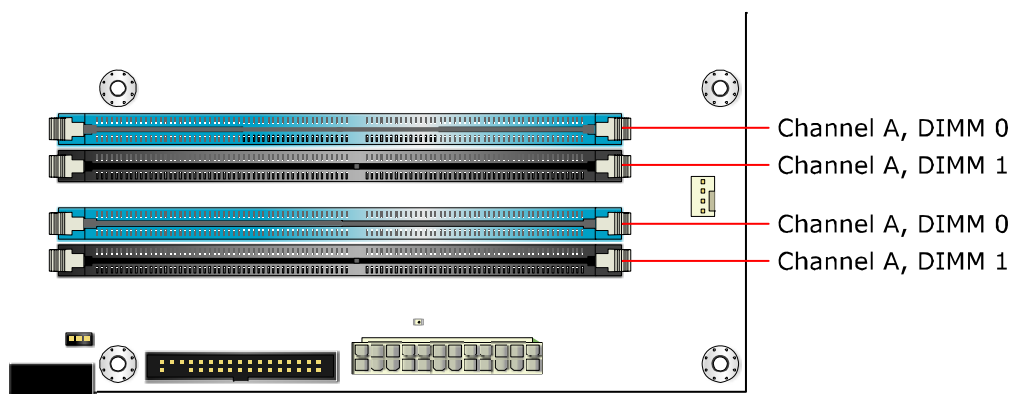
Figure 3. Memory Channel and DIMM Configuration
