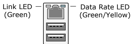
Figure 12. LAN Connector LED Locations
