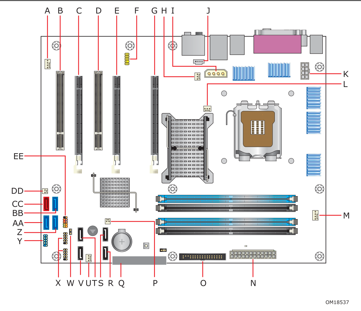
Figure 20. Component-side Connectors and Headers
