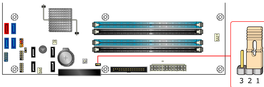
Figure 24. Location of the Jumper Block
