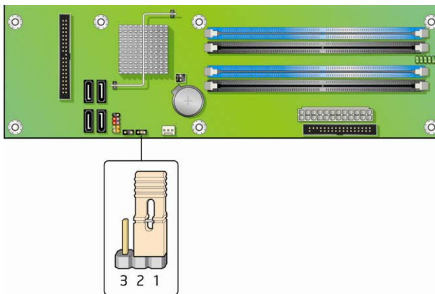
Figure 27. Location of the BIOS Configuration Jumper Block
