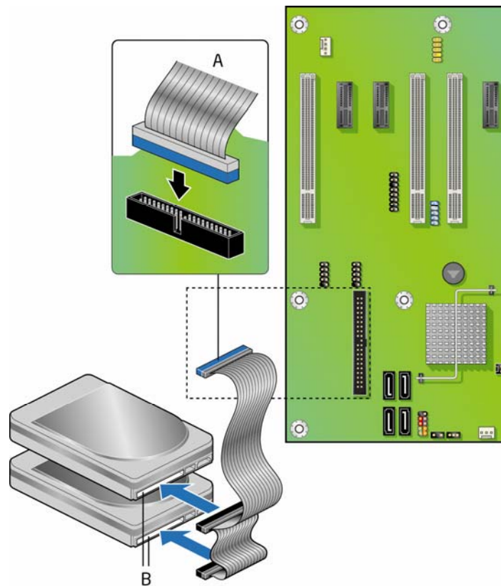
Figure 20. Connecting the IDE Cable
