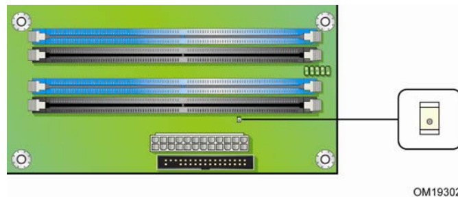
Figure 3. Location of Standby Power Indicator
