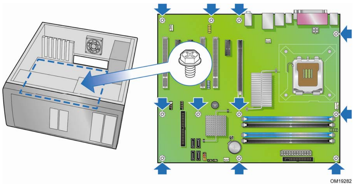
Figure 5. Desktop Board DG965RY Mounting Screw Hole Locations
