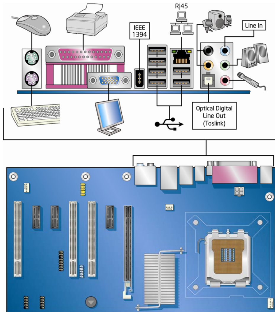
Figure 28. Back Panel Connectors
