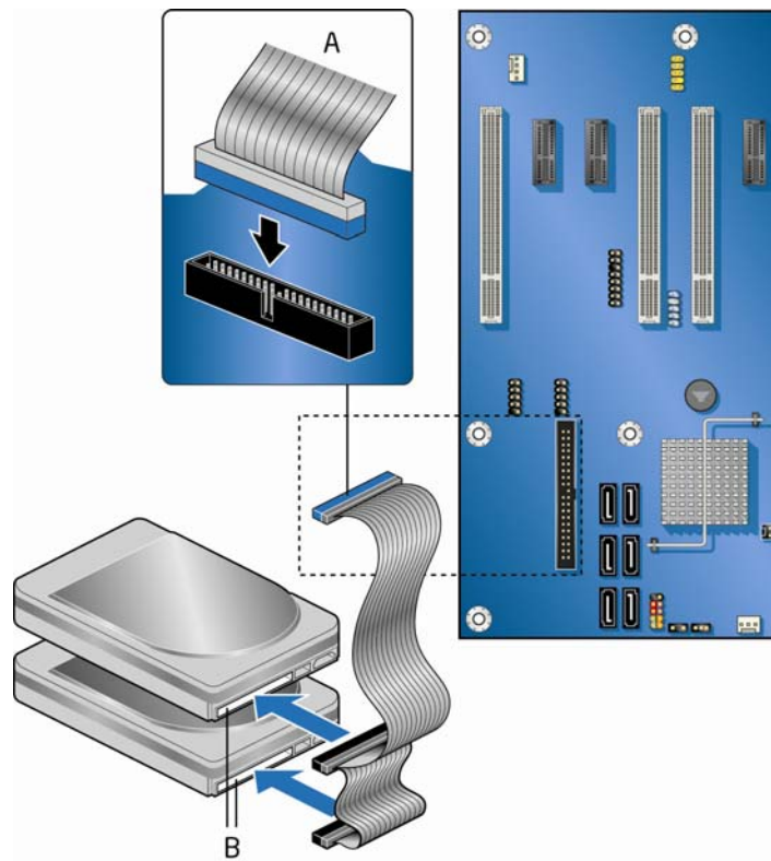
Figure 20. Connecting the IDE Cable
