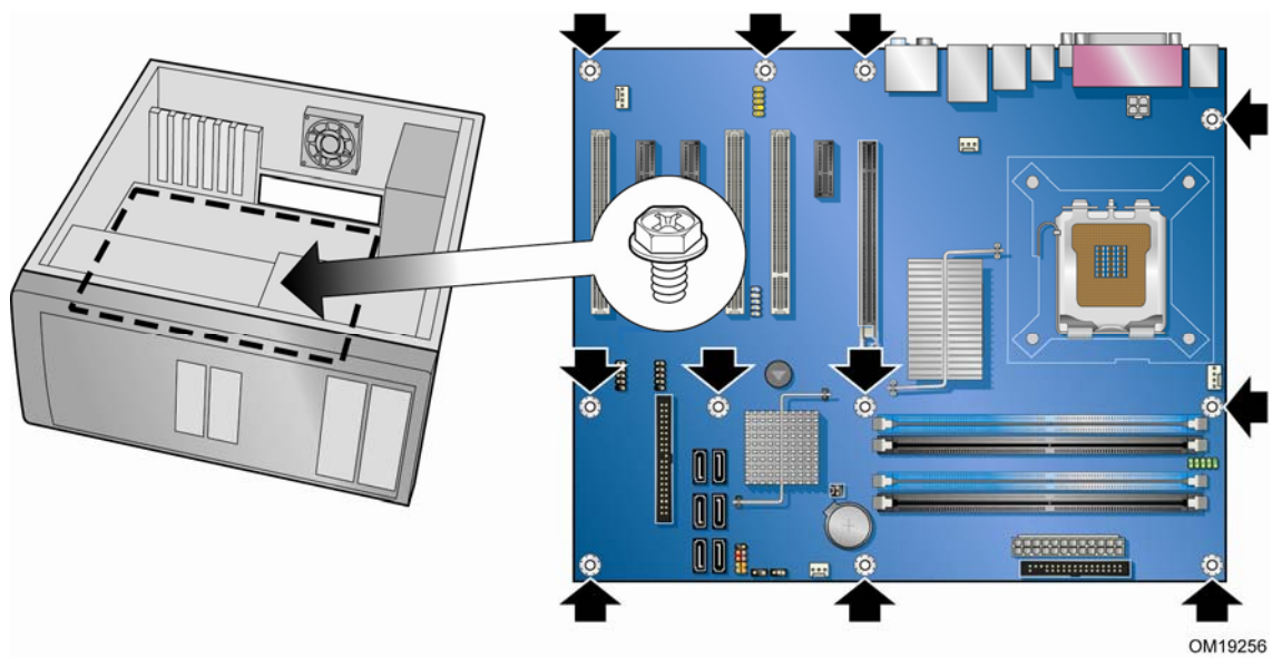
Figure 5. Desktop Board DG965WH Mounting Screw Hole Locations
