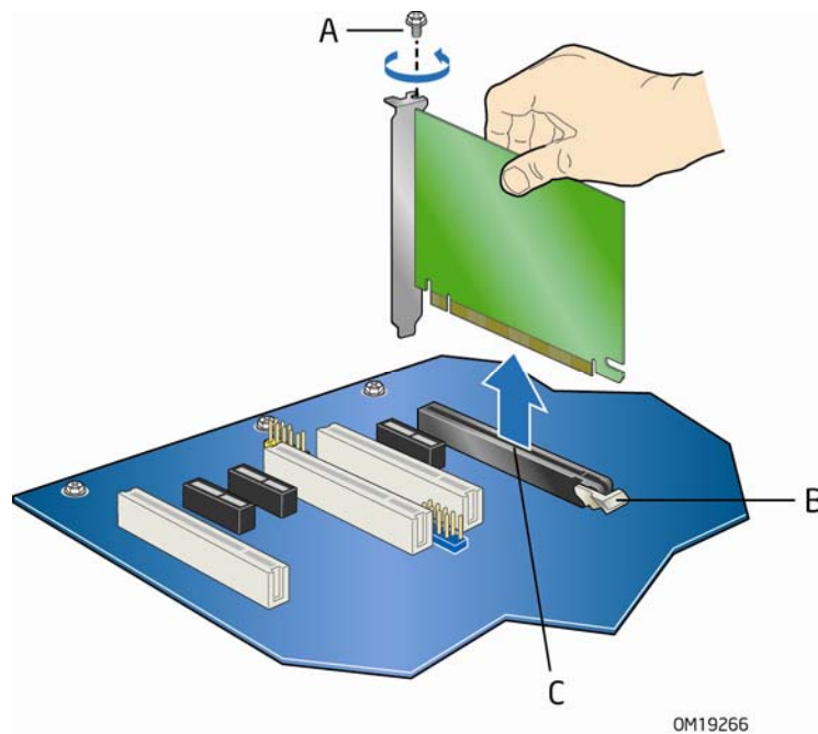
Figure 19. Removing a PCI Express x16 Card
