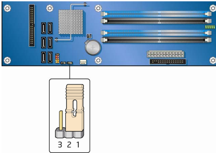
Figure 27. Location of the BIOS Configuration Jumper Block
