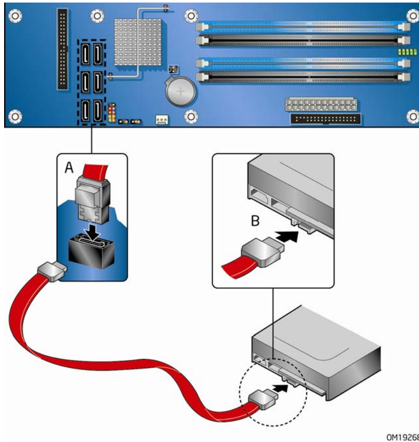
Figure 21. Connecting the Serial ATA Cable
