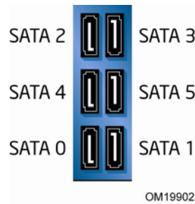
Figure 31. SATA Port Mapping for Desktop Board DG965WH After RAID is Enabled
