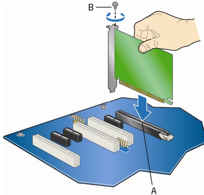
Figure 18. Installing a PCI Express x16 Card
