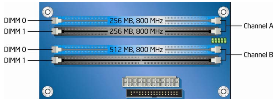
Figure 15. Dual Channel Memory Configuration Example 3
