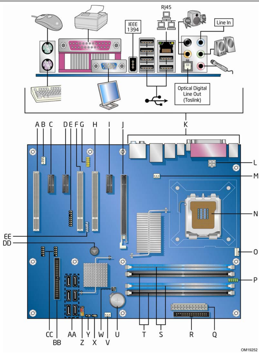
Figure 1. Desktop Board DG965WH Components
