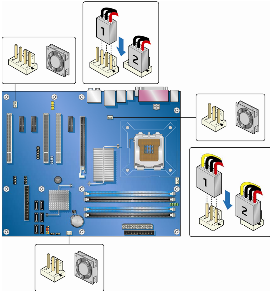
Figure 24. Location of Chassis Fan Headers
