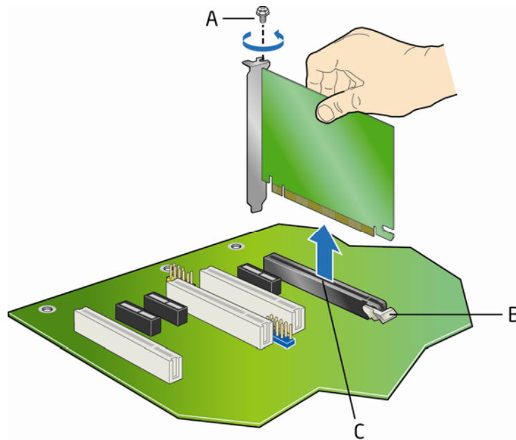
Figure 19. Removing a PCI Express x16 Card
