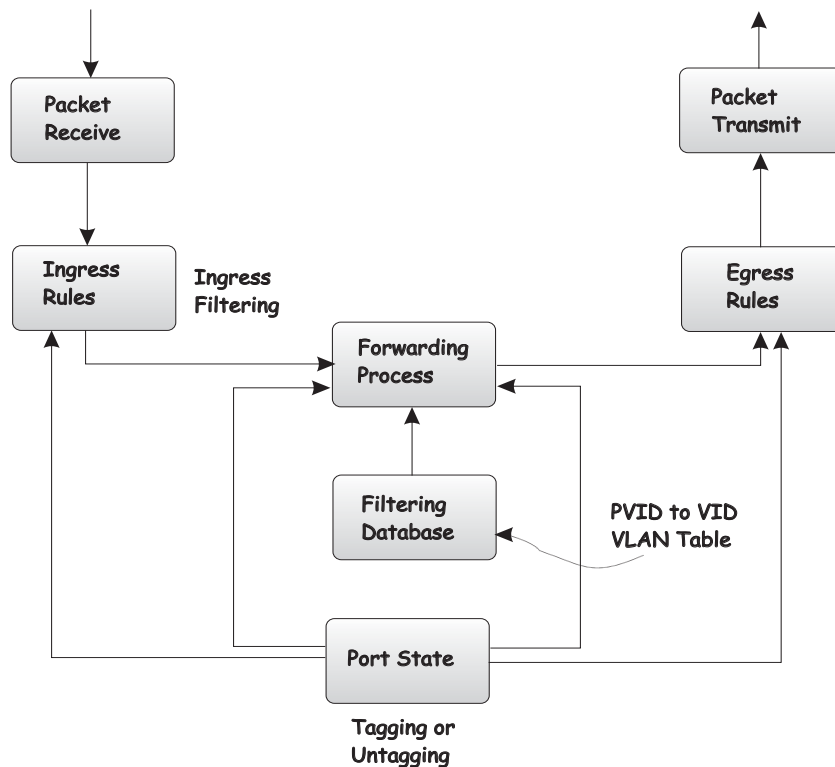
802.1Q Packet Forwarding
