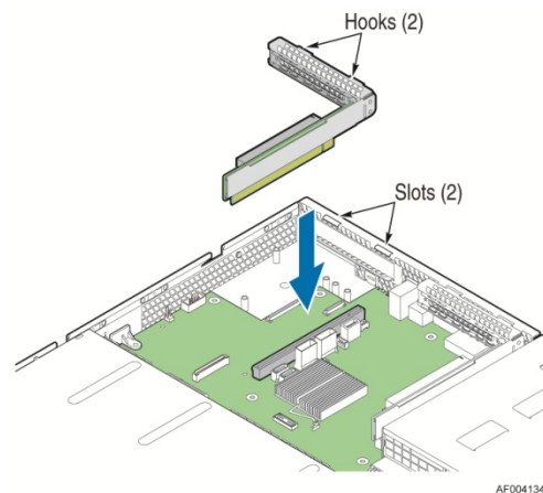
Figure 45. Add-in Card Support
