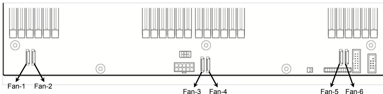
Figure 16. Server Board System Fan Connector Locations
