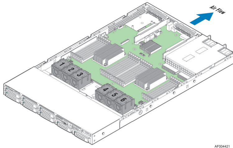
Figure 15. System Fan Identification
