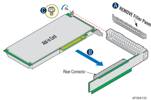
Figure 46. Riser Card Assembly
