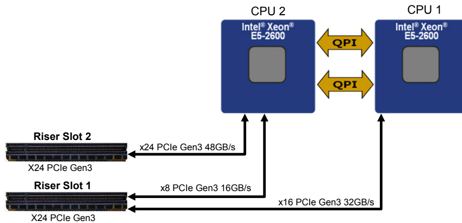
Figure 44. Riser Slot Architecture
