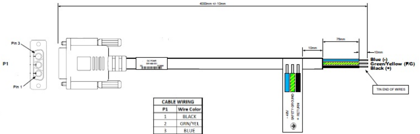
Figure 14. DC Power Cord
