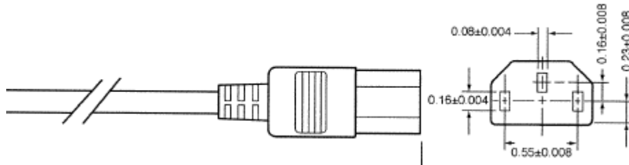
Figure 13. AC Power Cord
