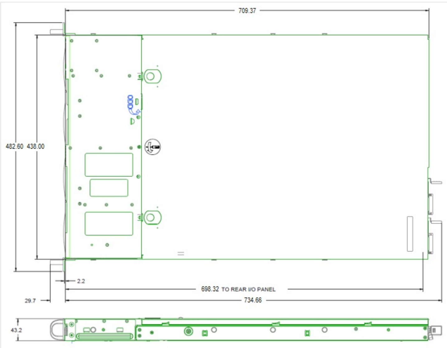
Figure 1. Chassis Dimensions
