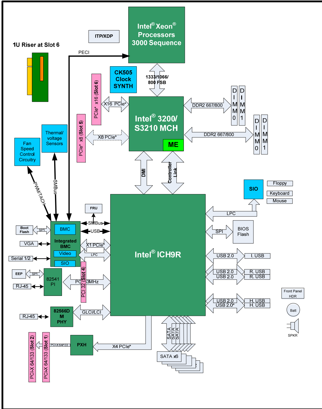
Figure 8. Intel® Server Systems S3200SH/S3210SH LX SKU-Block Diagram
