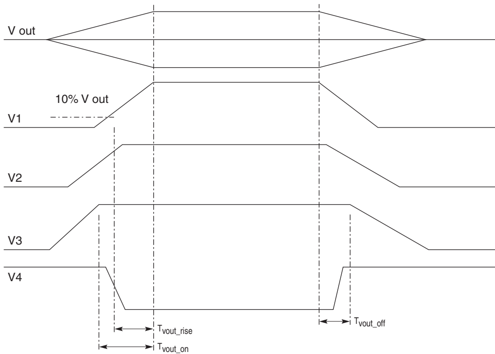
Figure 60. Output Voltage Timing
