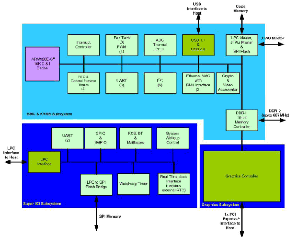
Figure 20. Integrated BMC Hardware
