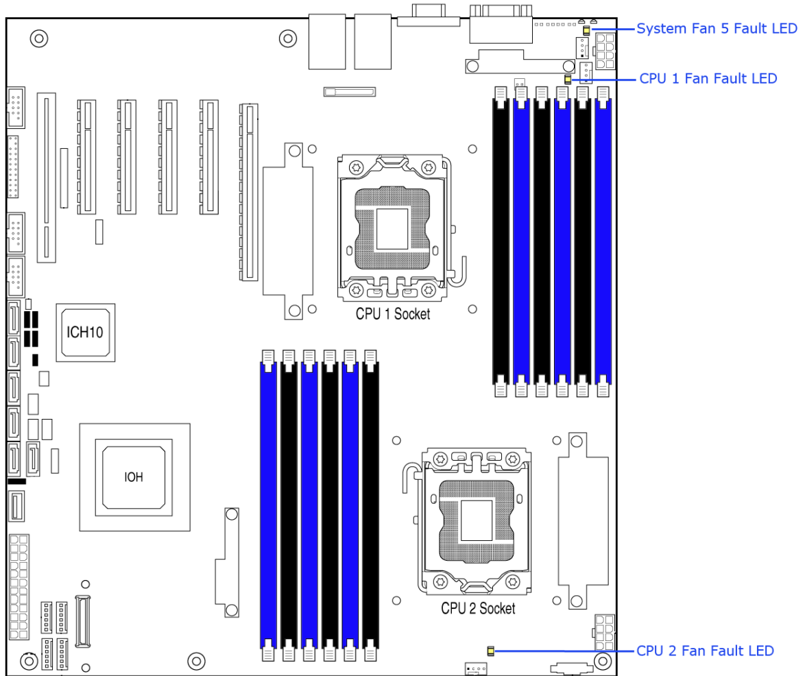
Figure 55. Fan Fault LED's Location
