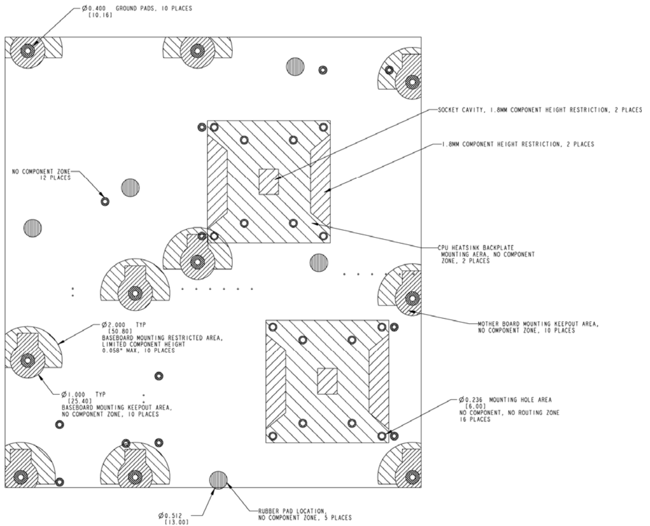
Figure 11. Second Side Keep-out Zone
