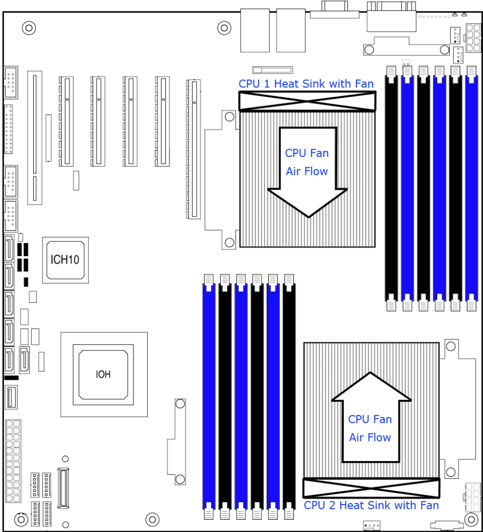
Figure 62. Active Processor Heatsink Installation Requirement
