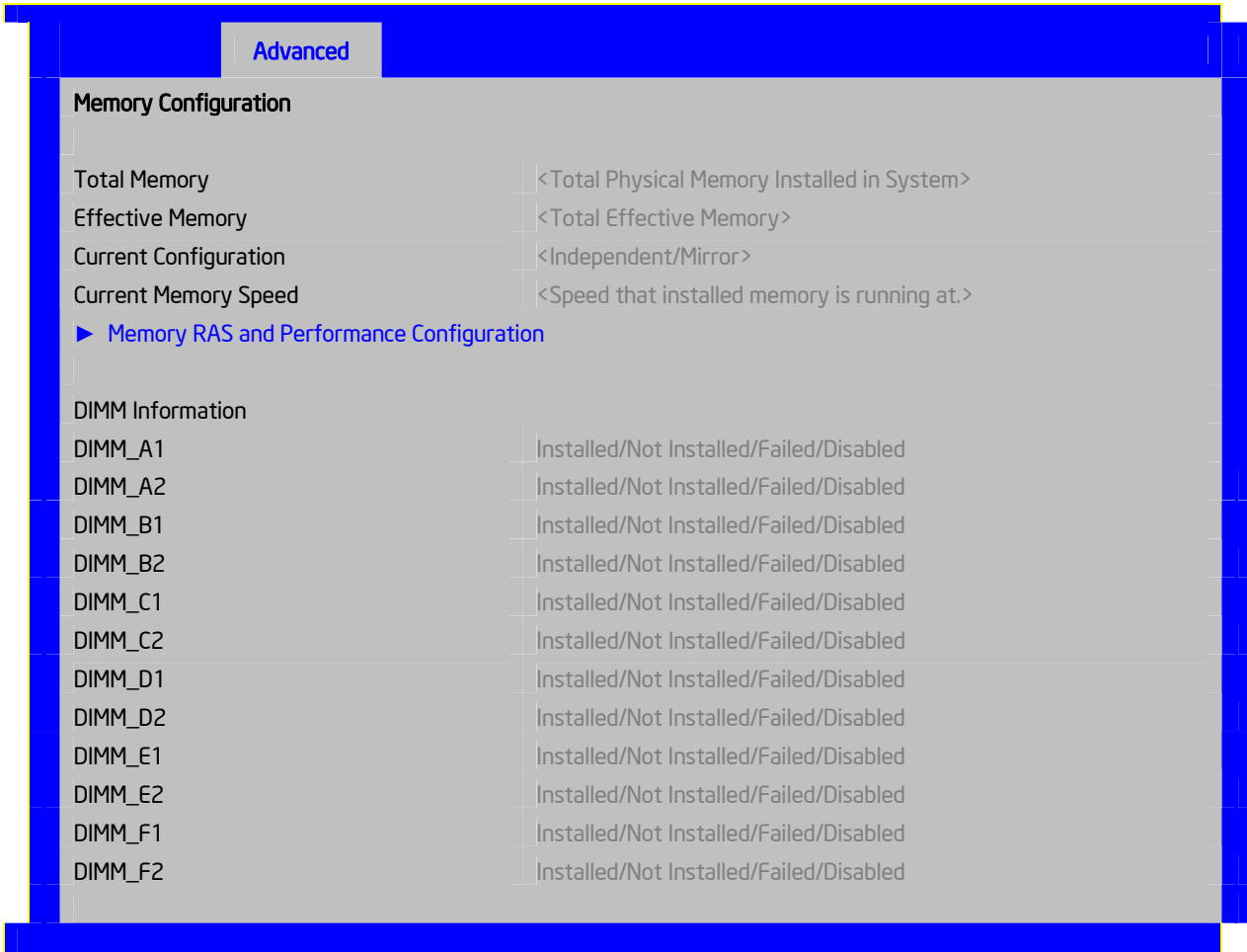
Figure 31. Setup Utility — Memory Configuration Screen Display
