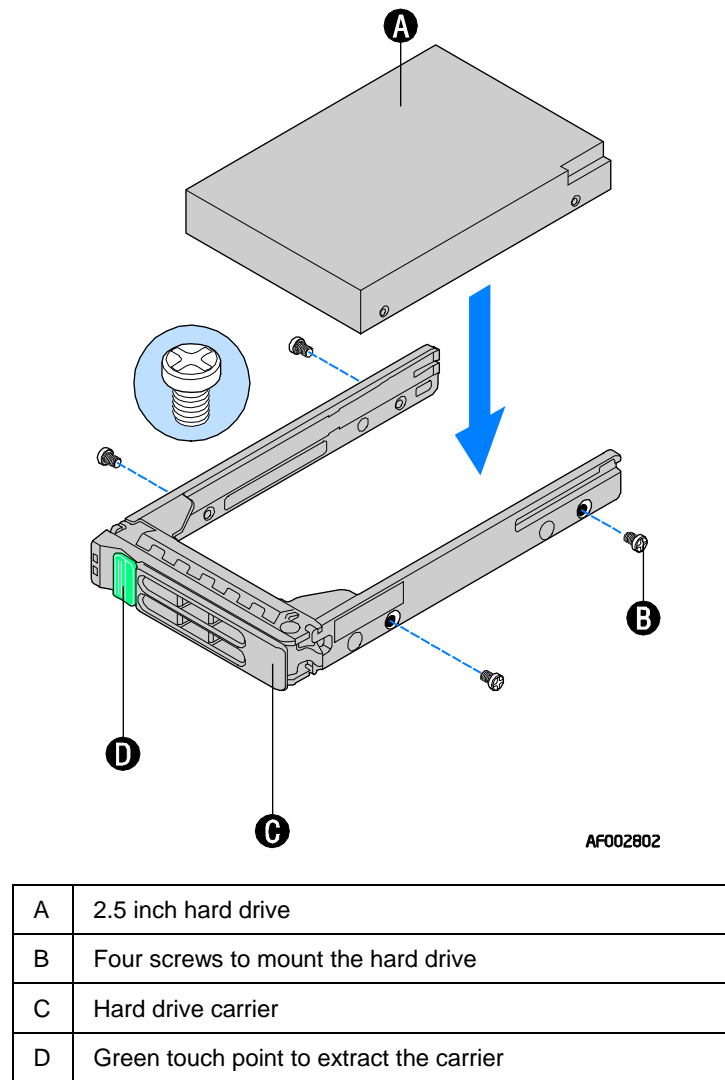
Figure 28. Hard Drive Tray Assembly
