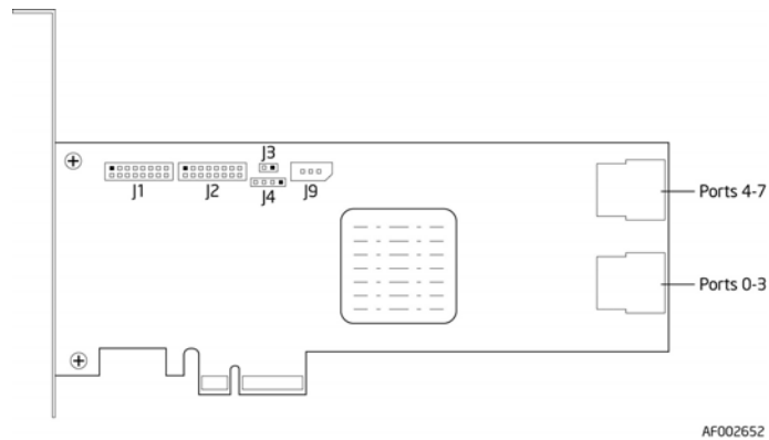
Figure 4. Card Layout
