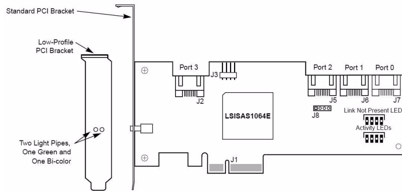
Figure 4. Card Layout
