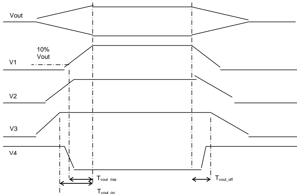
Figure 26. Output Voltage Timing
