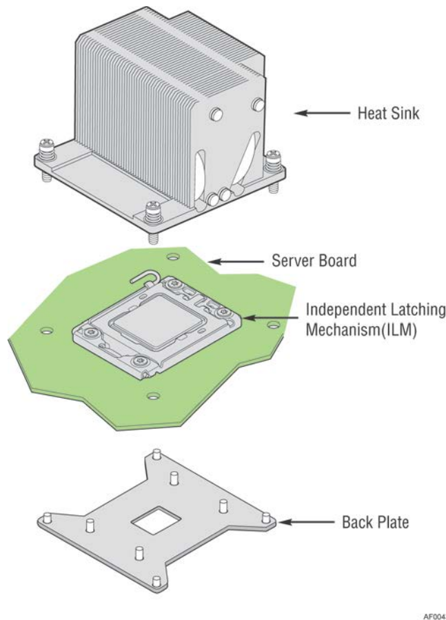
Figure 13. Processor Socket Assembly
