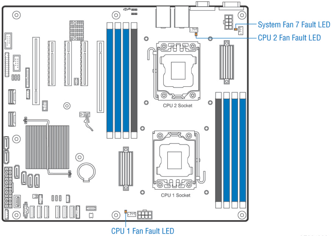
Figure 24. Fan Fault LED Locations
