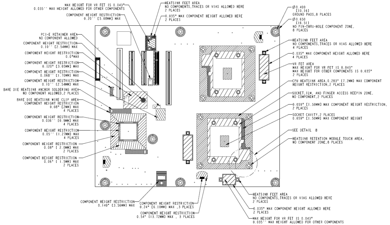
Figure 7. Intel® Server Boards S2400SC – Primary Side Keepout Zone
