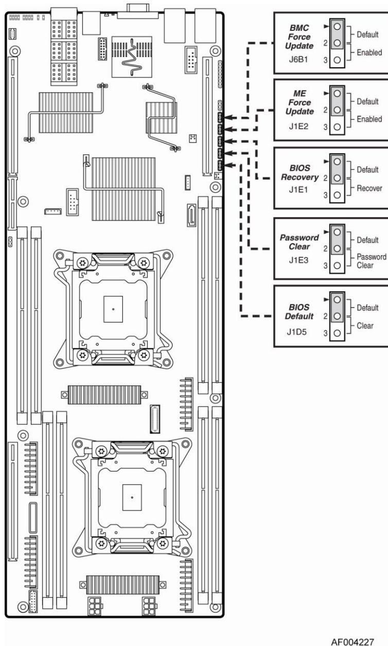
Figure 45. Jumper Blocks (J6B1, J1E2, J1E3, J1E1, J1D5)
