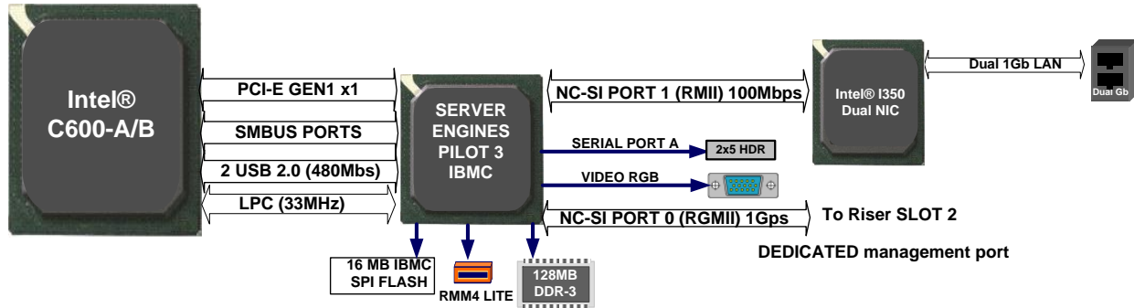
Figure 18. Integrated BMC implementation overview
