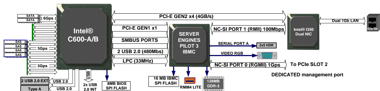
Figure 14. Intel® C600-A/B PCH connection
