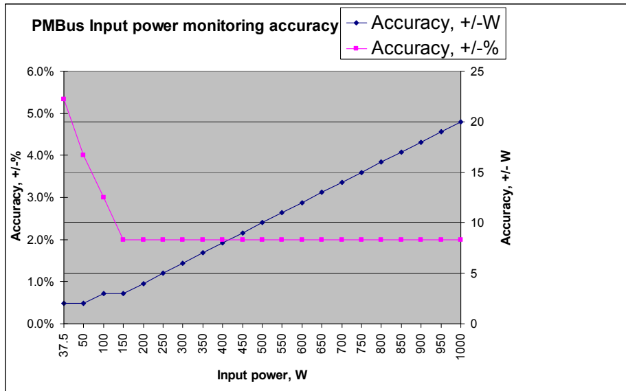
Figure 16. PMBus Monitoring Accuracy
