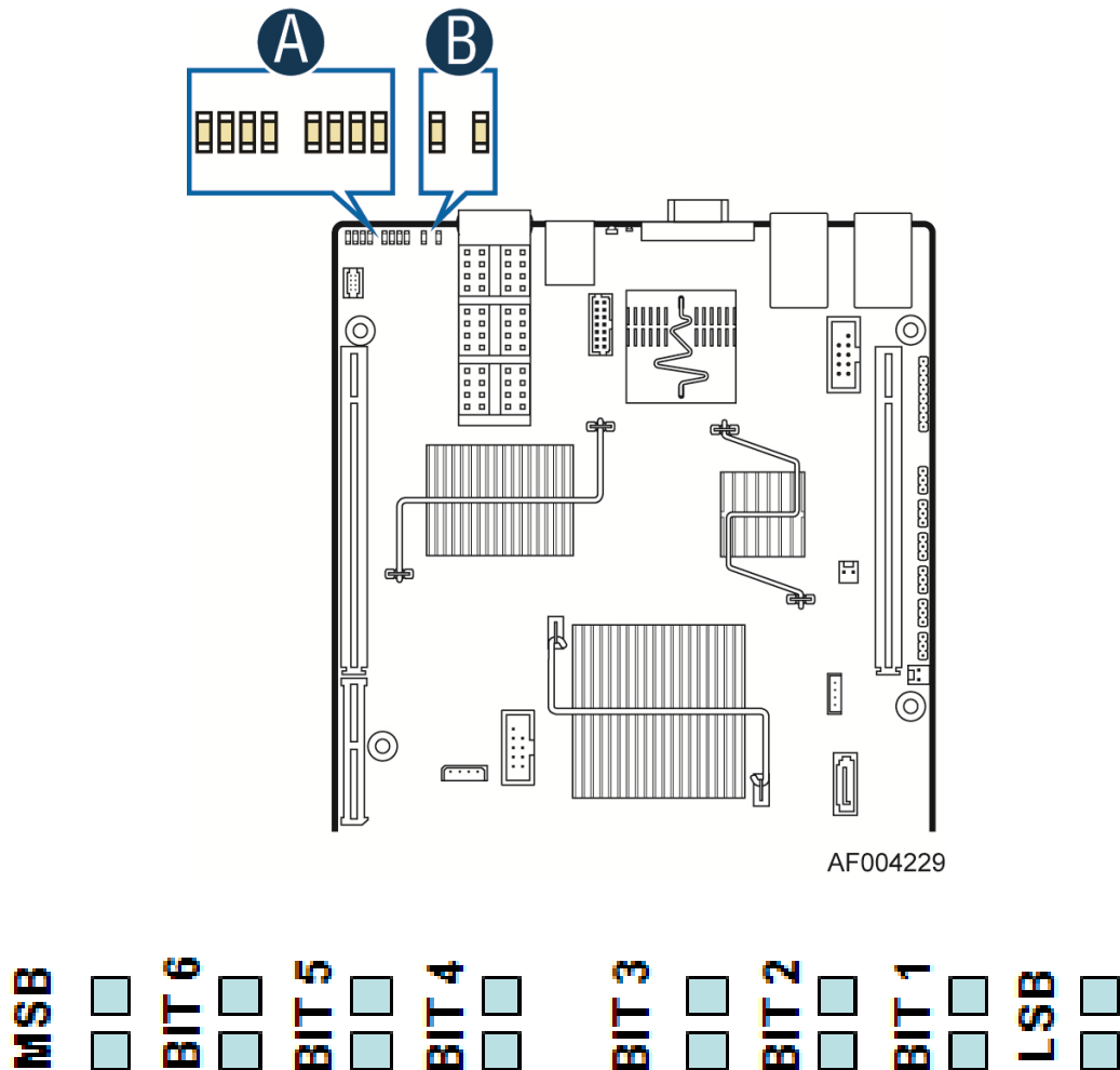
Figure 39. Diagnostic LED location
