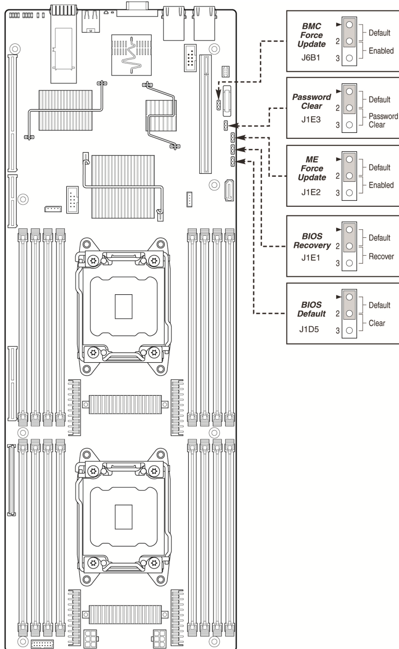
Figure 35. Jumper Locations and Functions
