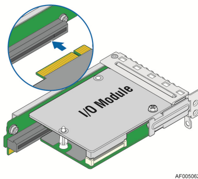
Figure 37. PCI Express Riser with bracket for Riser Slot 2
