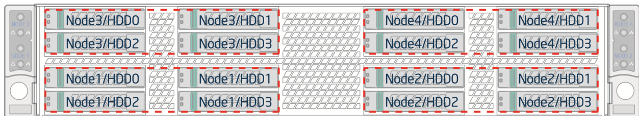
Figure 24. HDD Scheme for H2312WPGR
