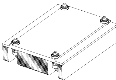
Figure 17. Processor Heatsink Overview
