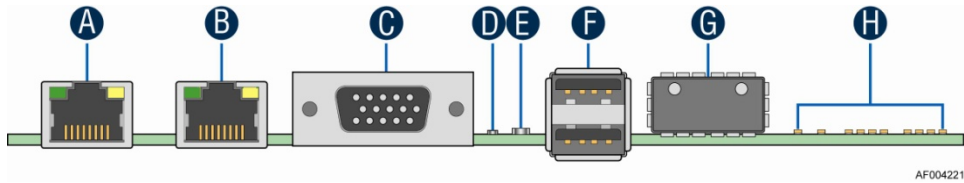
Figure 6. Intel® Server Board S2600WP Components
