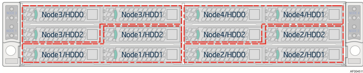
Figure 24. HDD Scheme for H2312WPGR
