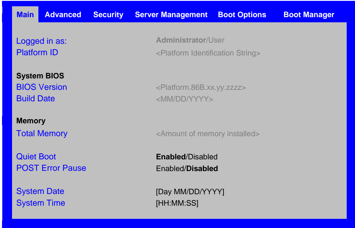
Figure 15. Main Screen
