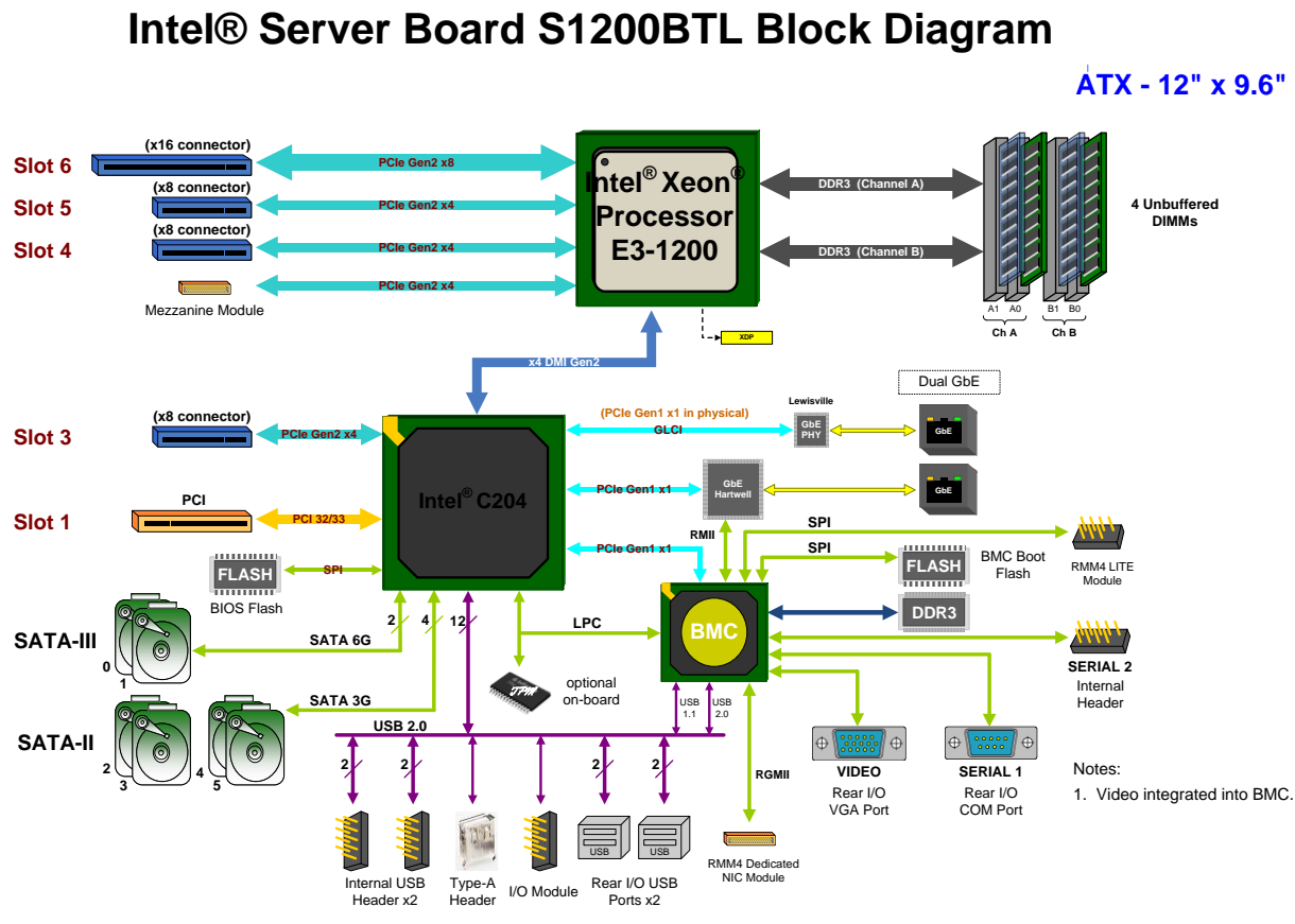
Figure 11. Intel® Server Board S1200BTL Functional Block Diagram
