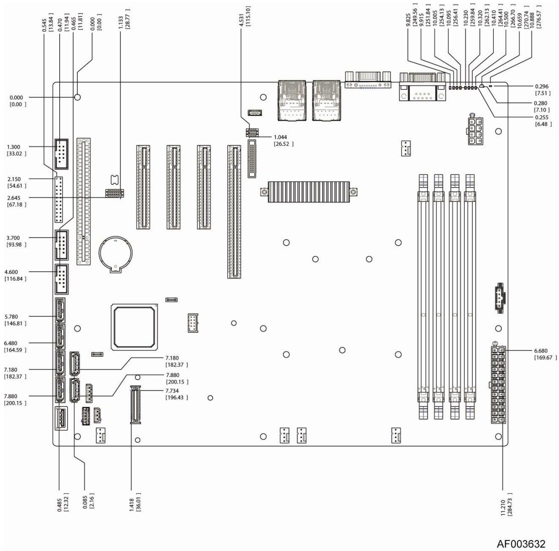
Figure 7. Intel® Server Board S1200BT – Major Connector Pin Location (2 of 2)
