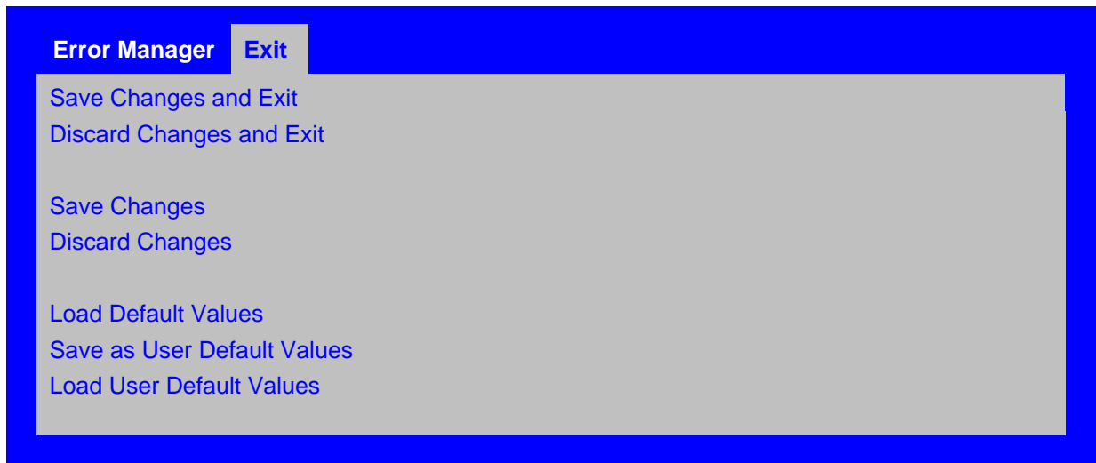
Figure 45. Exit Screen
