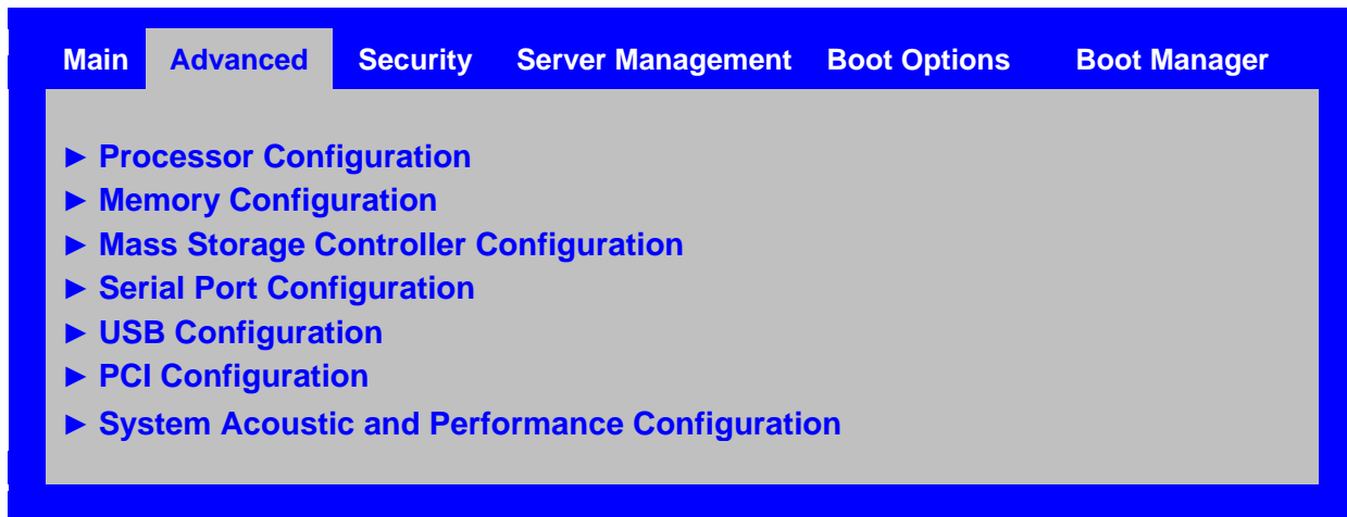
Figure 16. Advanced Screen
