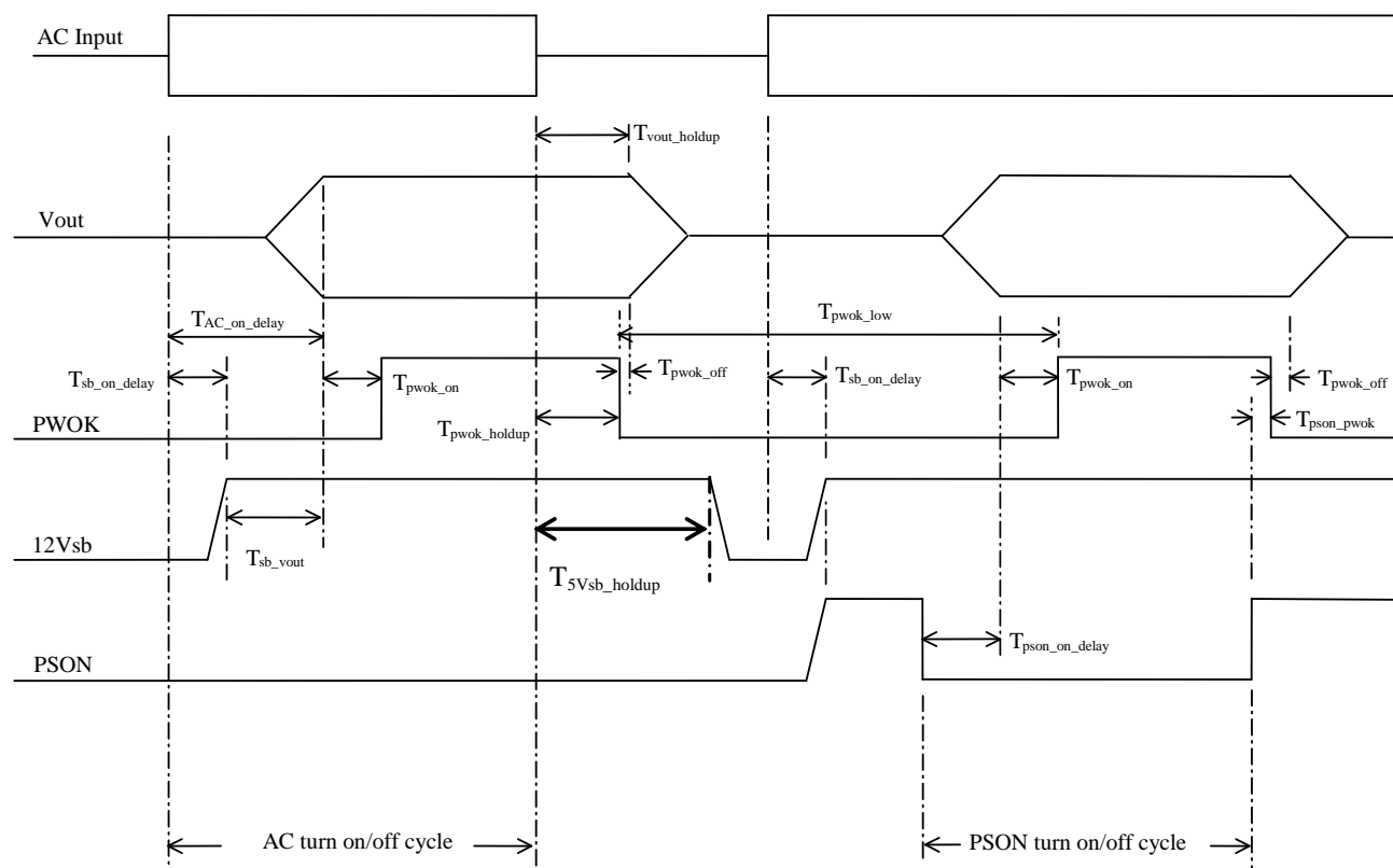
Figure 46. Turn On/Off Timing (Power Supply Signals)
