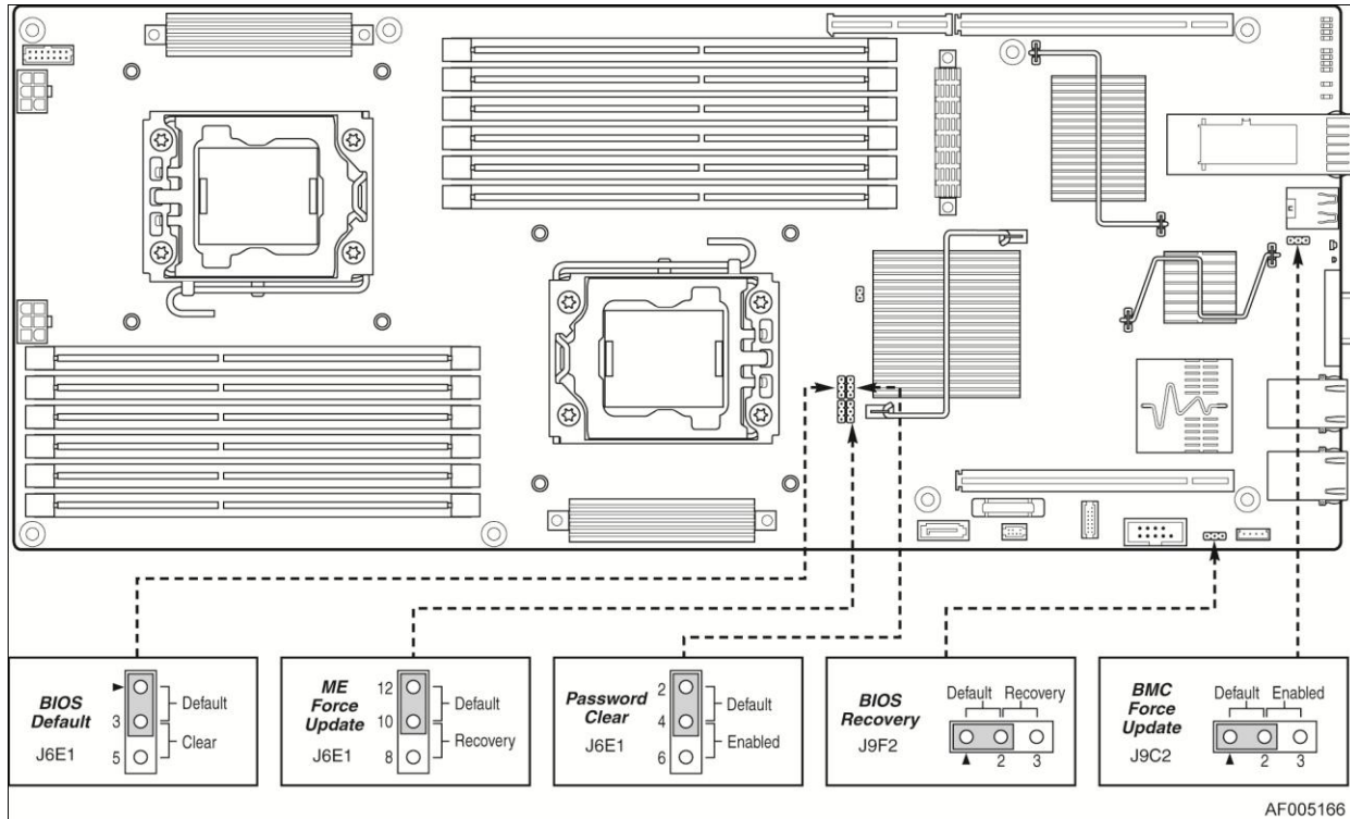
Figure 43: Jumper Blocks (J9C2, J9F2, J6E1, J6E1, J6E1, J6E1)
