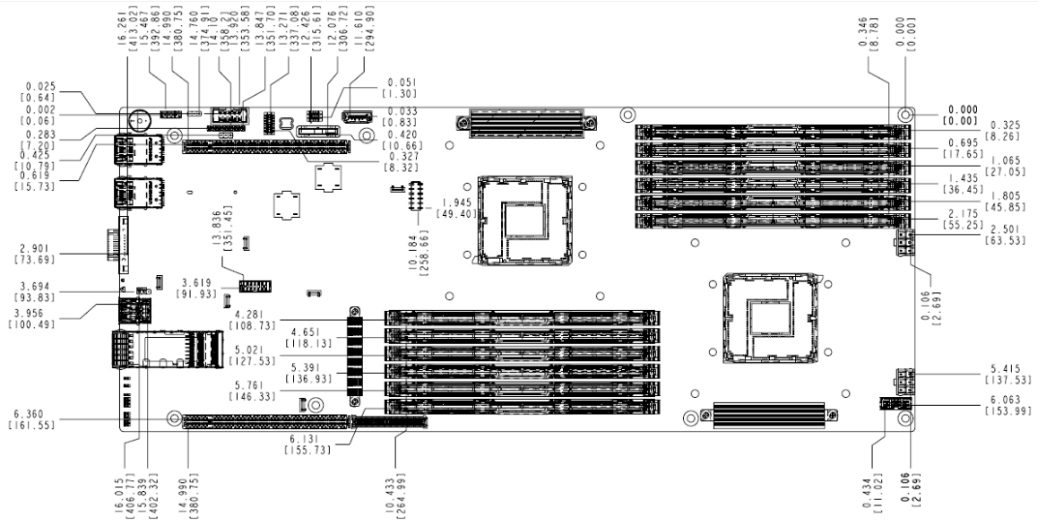
Figure 5. Intel® Server Boards S2400LP – Major Connector Pin-1 Locations
