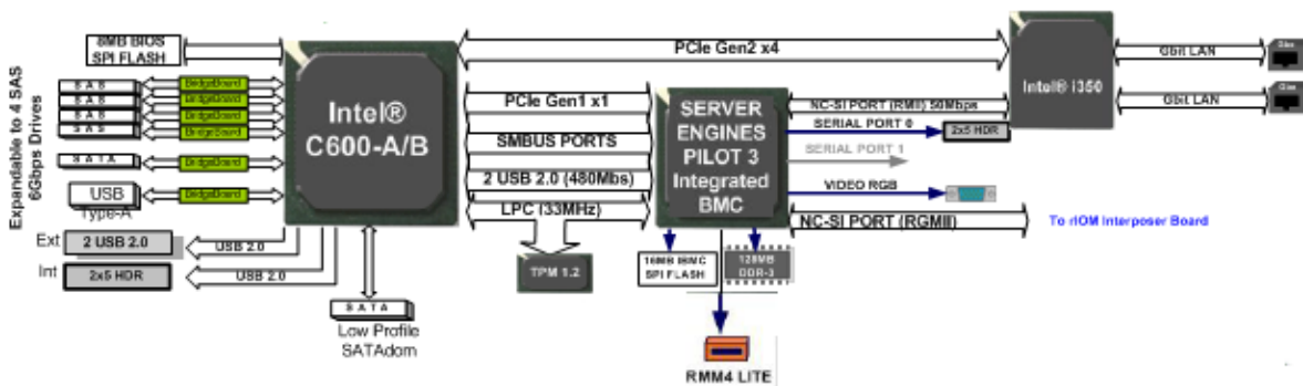
Figure 12. Intel® C600-A/B PCH connection
