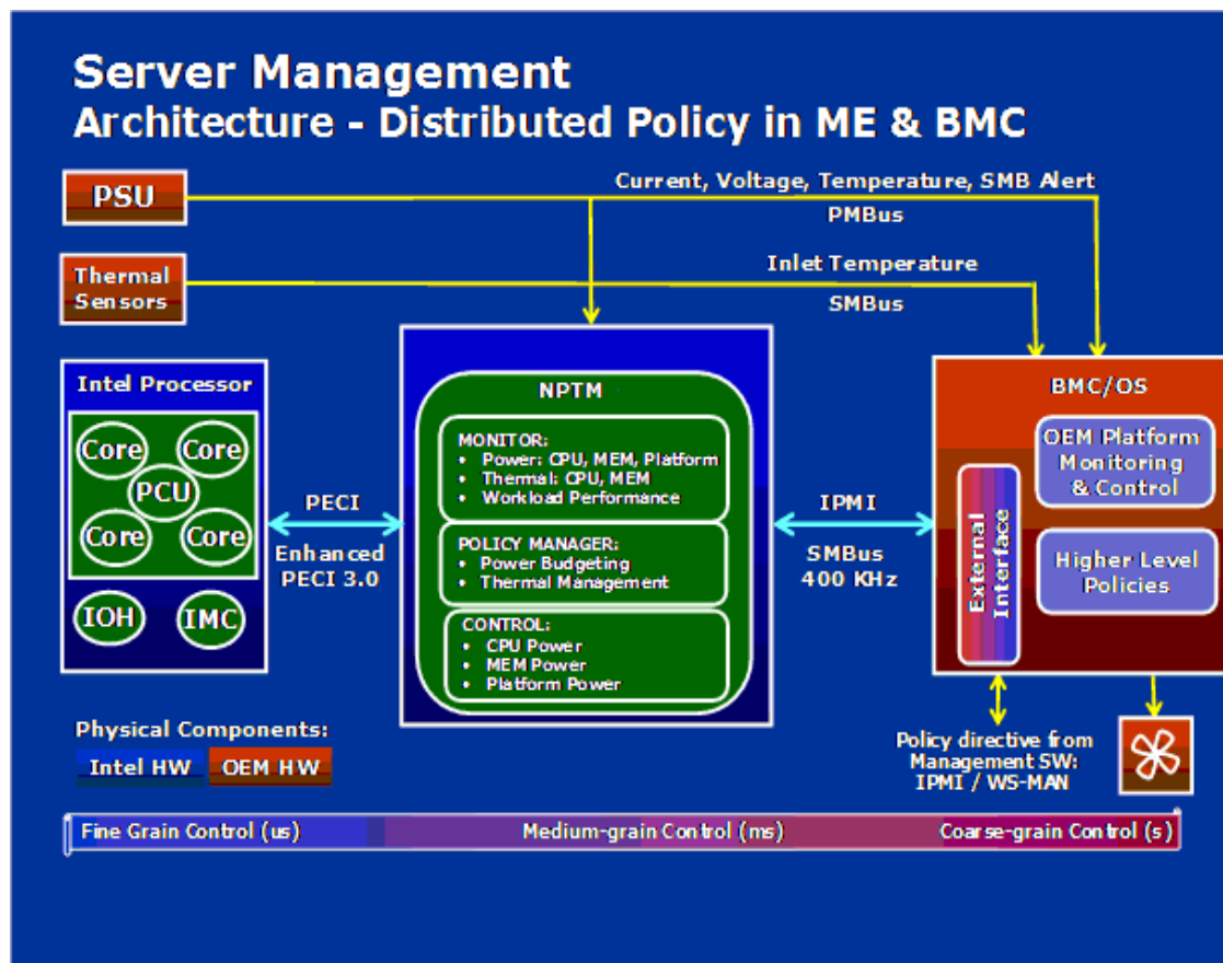
Figure 18. Management Engine Distribution Model
