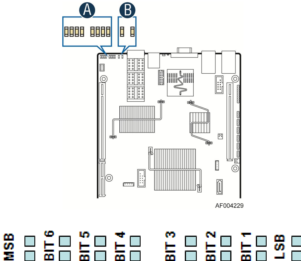
Figure 47. Diagnostic LED Placement Diagram
