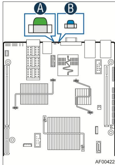
Figure 44. System Status LED (A) and ID LED (B)
