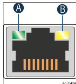
Figure 13. 1GbE NIC port LED
