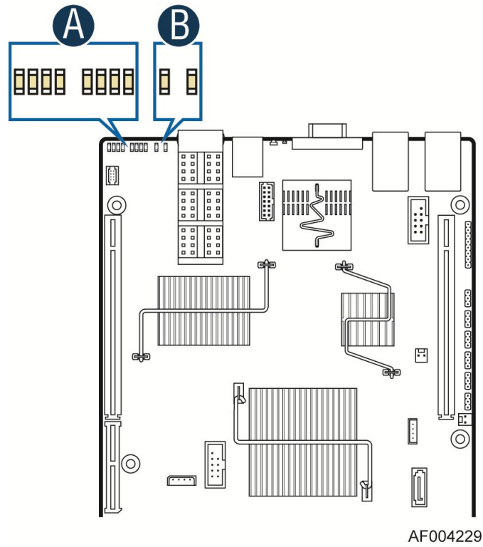
Figure 45. Rear Panel Diagnostic LEDs (Block A)
