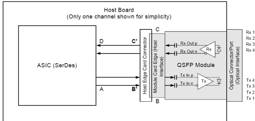
Figure 15. Connection between ConnectX®-3 and QSPF
