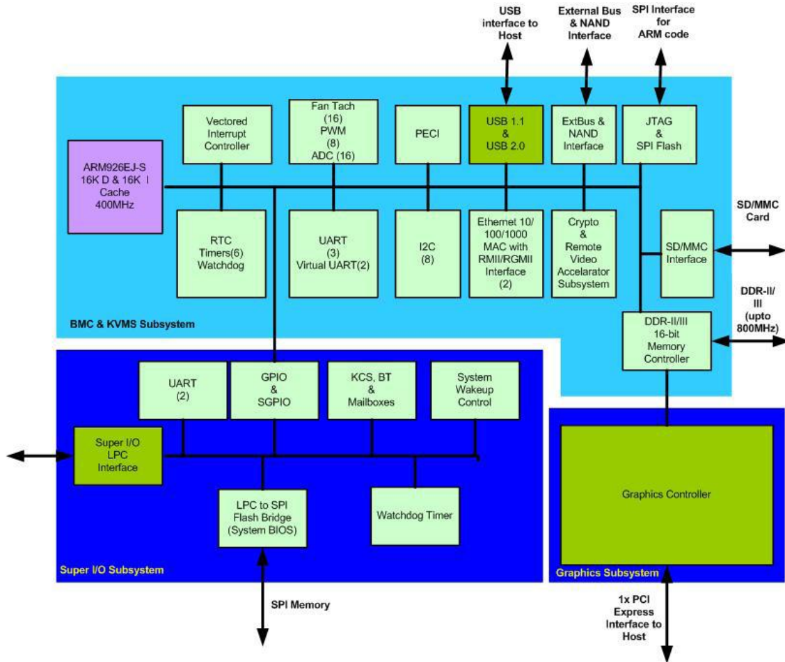
Figure 17. BMC Functional Block Diagram
