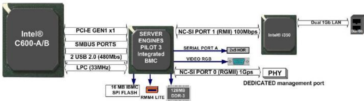
Figure 16. Integrated BMC implementation overview
