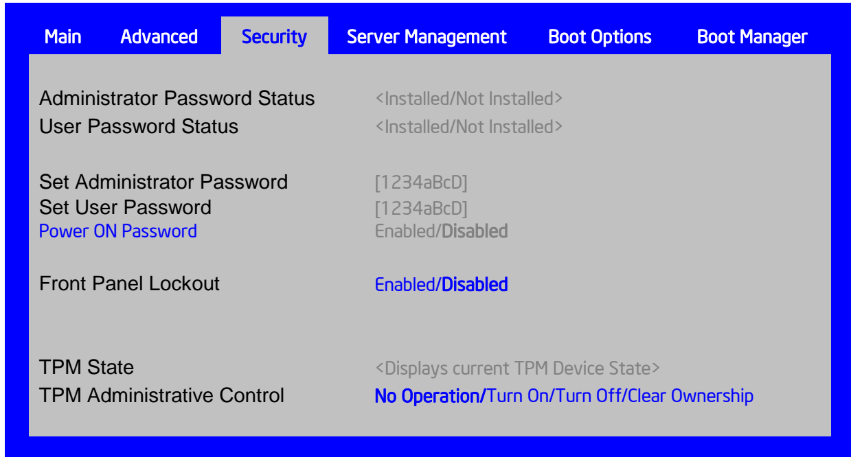
Figure 24. Security Screen
