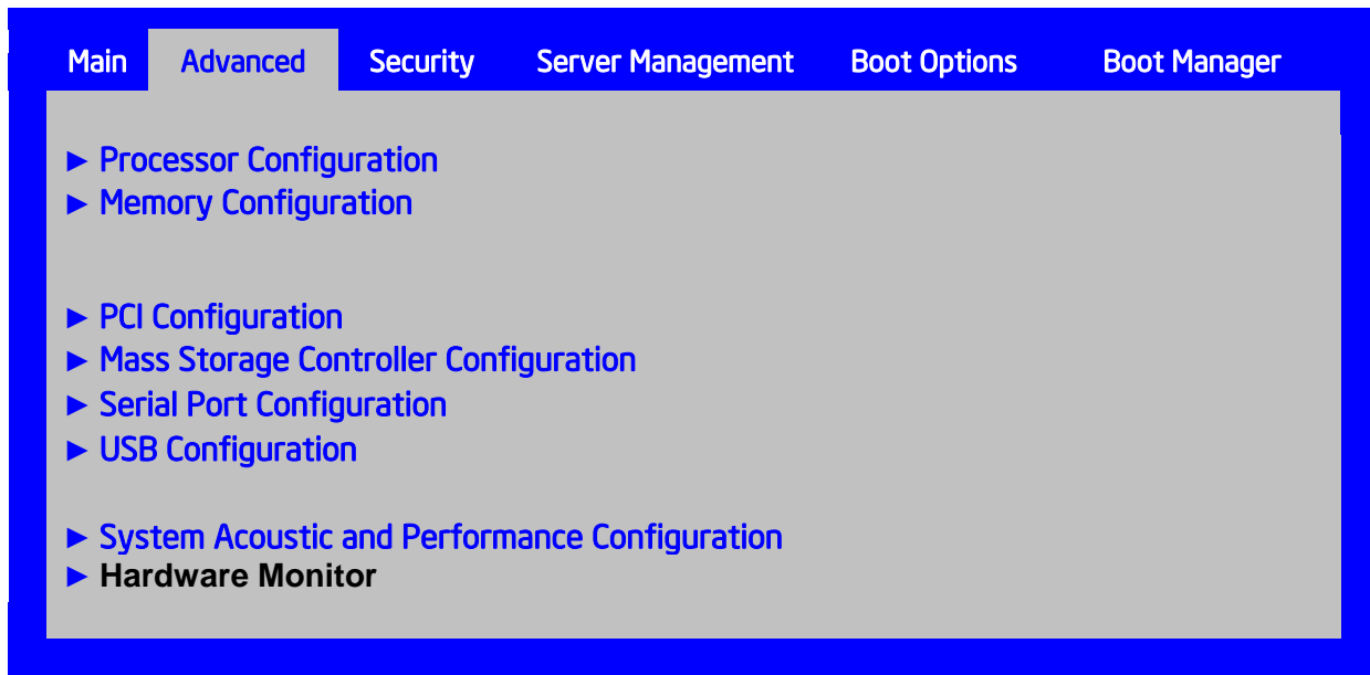
Figure 16. Advanced Screen
