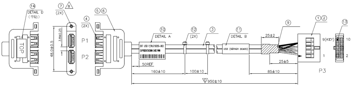
Figure 24. USB Cable Drawing
