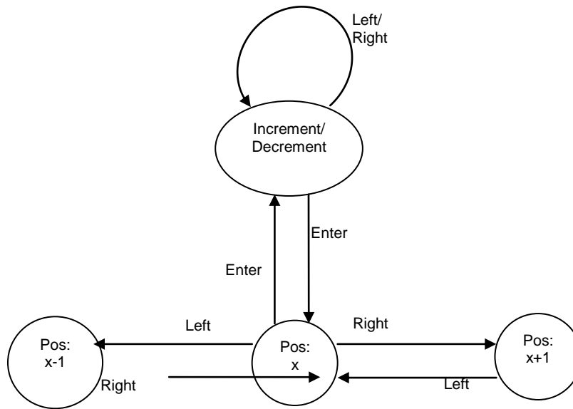
Figure 59. State transition diagram for setting IP Address
