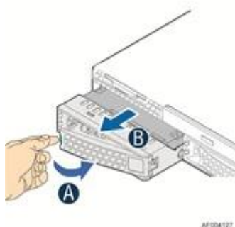
Figure 29. Removing 3.5" Hard Disk Drive
