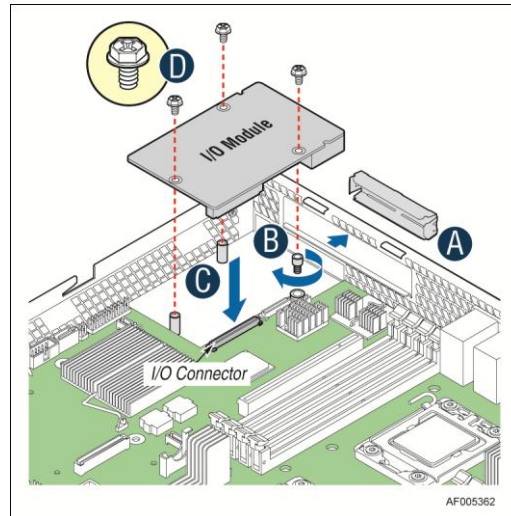
Figure 64. Installing I/O Module
