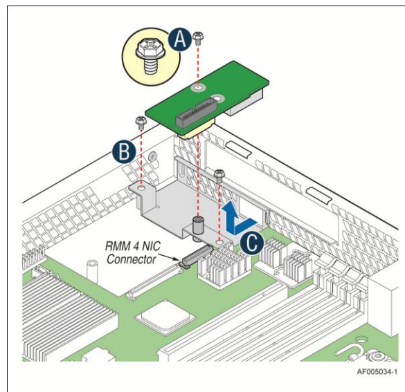
Figure 66. Intel® RMM4 Dedicated Management NIC Installation
