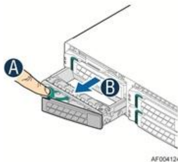
Figure 23. Removing 2.5" Hard Disk Drive
