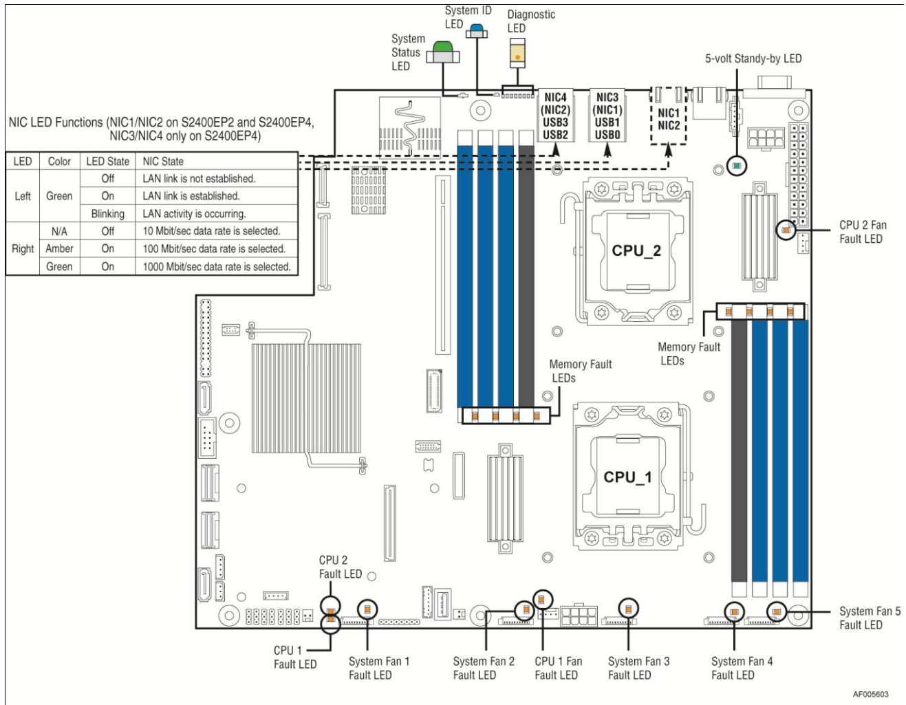
Figure 10. Intel® Light-Guided Diagnostic LEDs - Server Board
