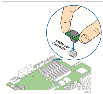
Figure 37. Installing RMM4 Lite Figure
