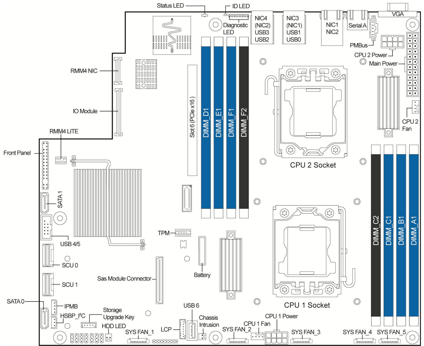
Figure 9. Intel® Server Board S2400EP
