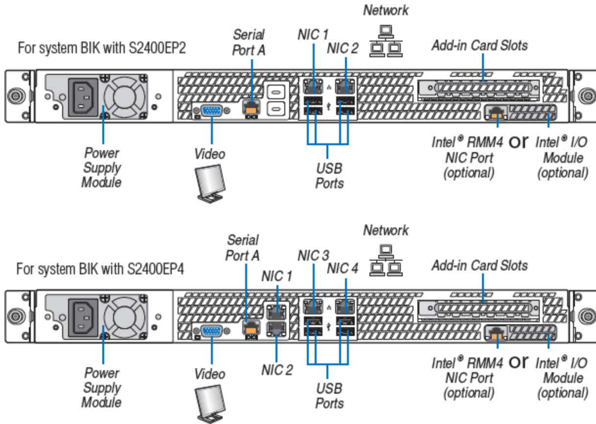
Figure 7. Back Panel Feature Identification
