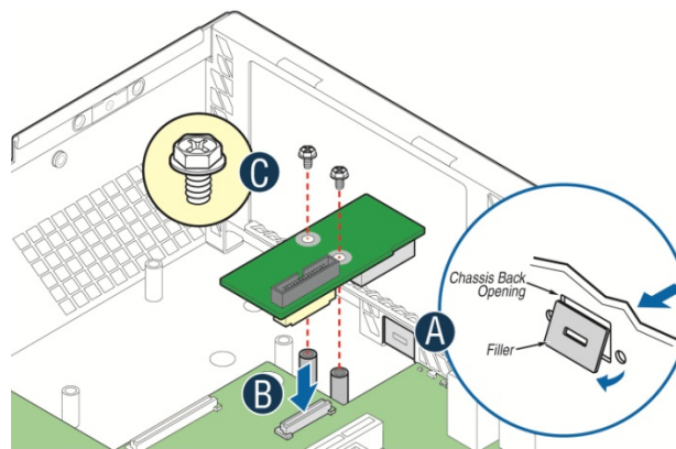
Figure 49. Intel® RMM4 Lite Activation Key Installation
