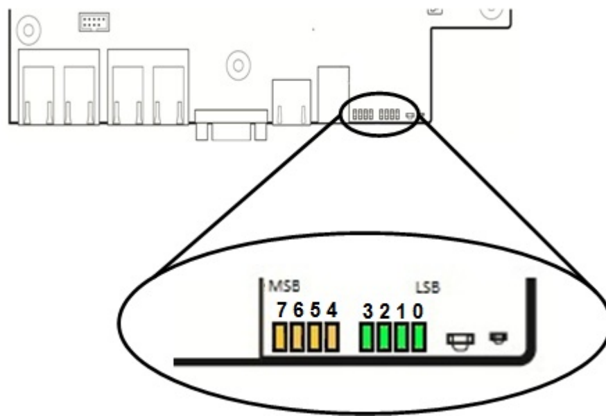
Figure 51. POST Diagnostic LED Location
