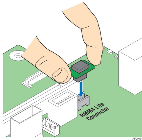
Figure 49. Intel® RMM4 Lite Activation Key Installation
