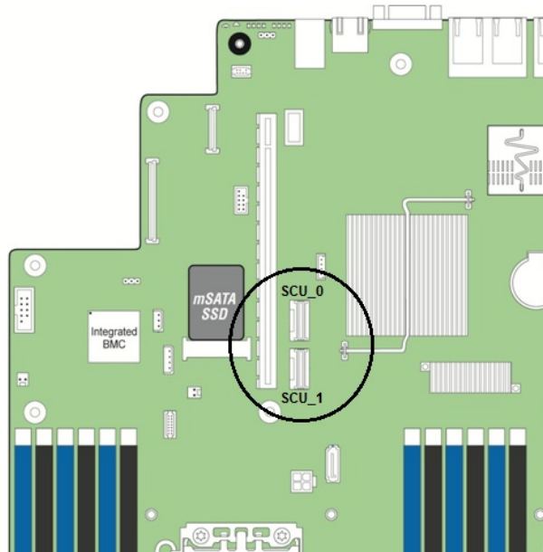
Figure 22. SCU Ports
