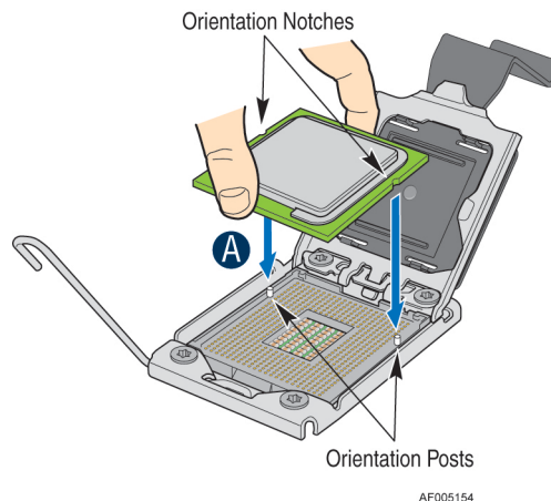
Figure 8. Processor Installation
