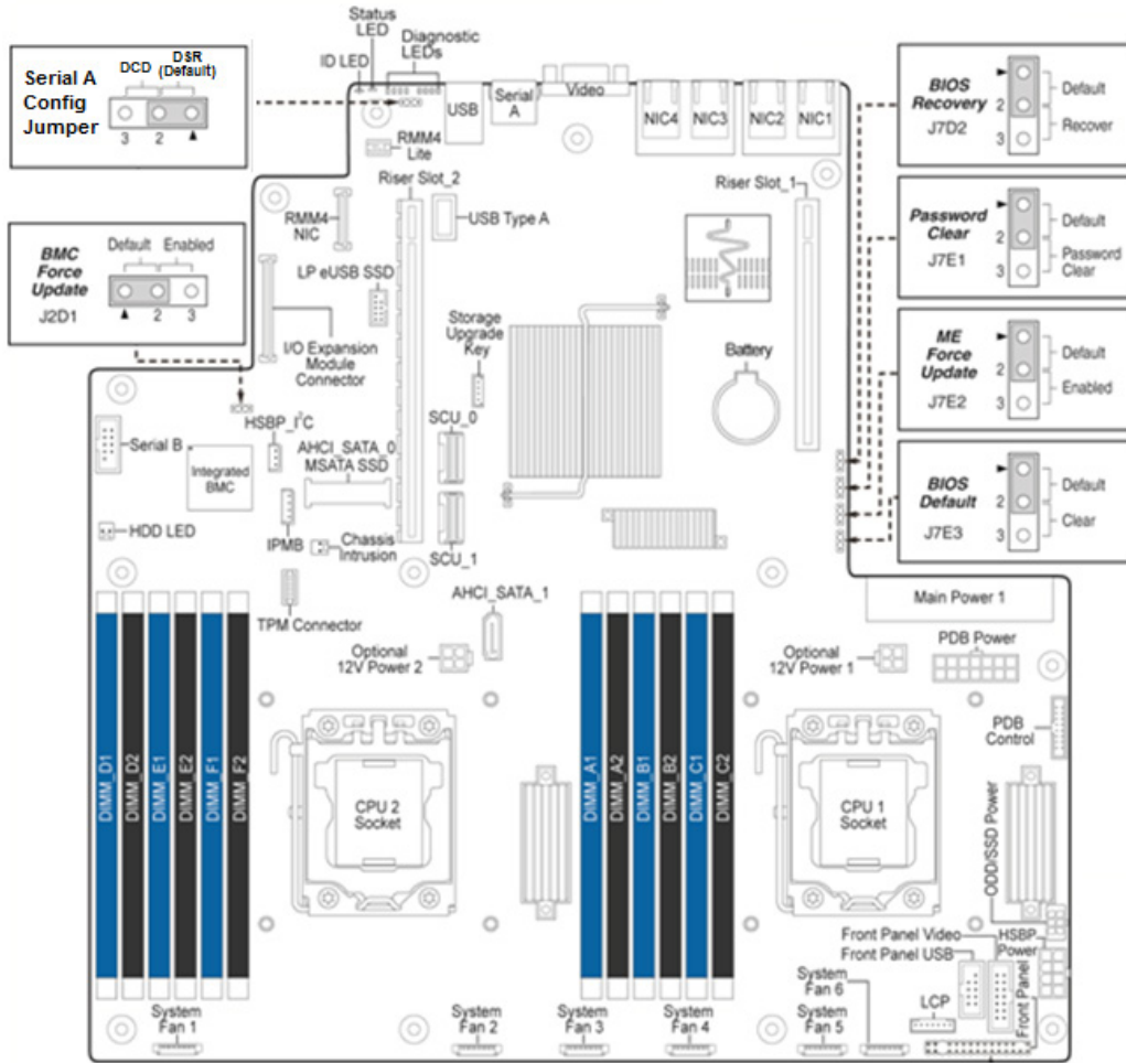
Figure 4. Jumper Block Identification
