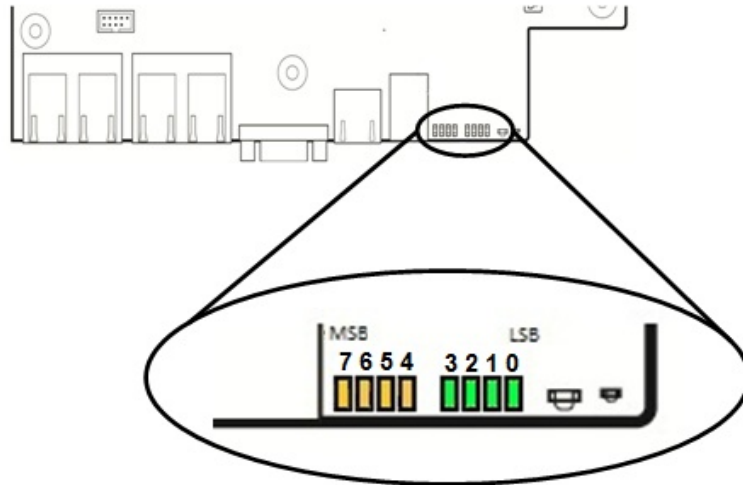
Figure 34. POST Diagnostic LED Location
