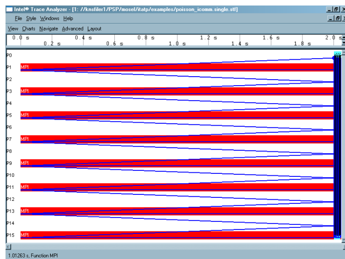
Figure 4-5. Event Timeline: Use Available Vertical Space checked
