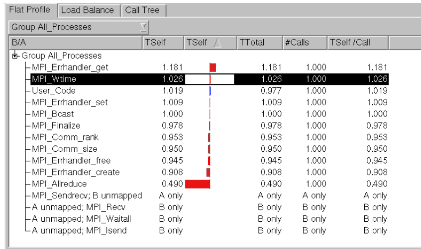
Figure 6-5. A Comparison Function Profile Chart
