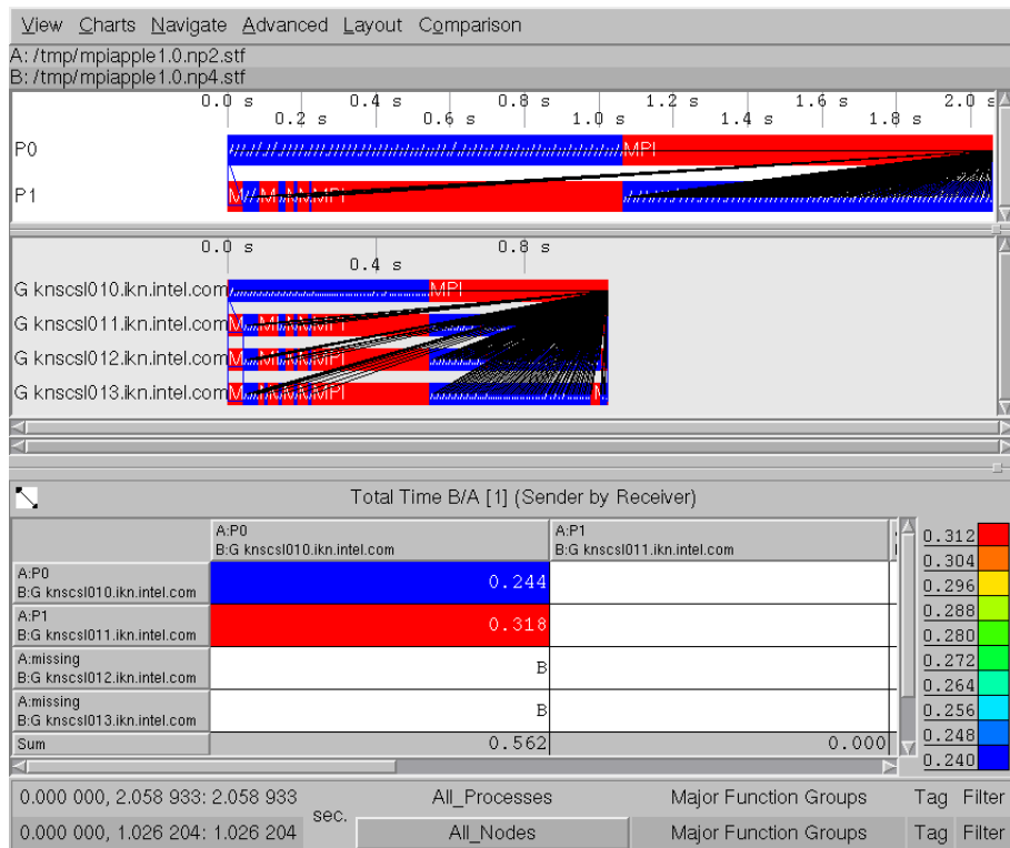
Figure 6-8. The Comparison Message Profile
