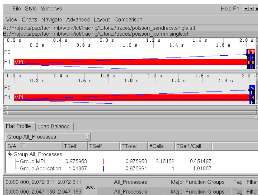
Figure 6-1. A comparison View
