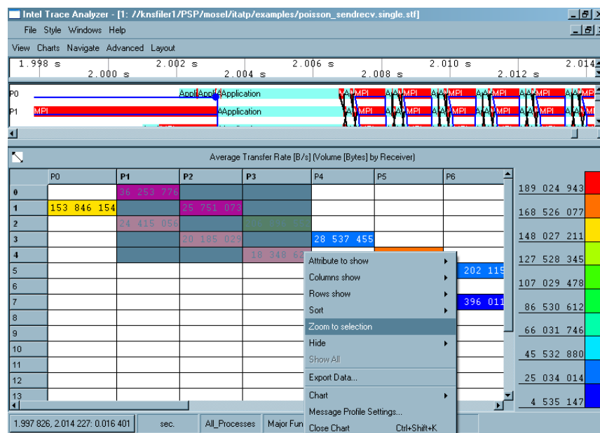
Figure 4-43. Selecting an area in the matrix and zooming into
