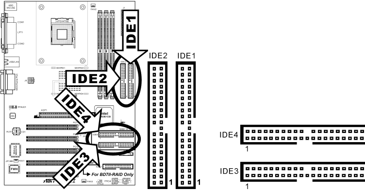
40 Pin IDE Plug On The Motherboard Blue Connector
