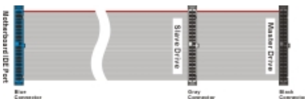
Figure 2-10. Nappe Ultra DMA 66
