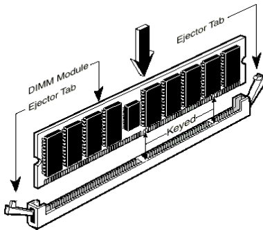
Figure 2-6. Memory module installation
