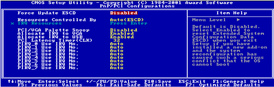
Figure 3-9. Menu du PnP/PCI Configurations
